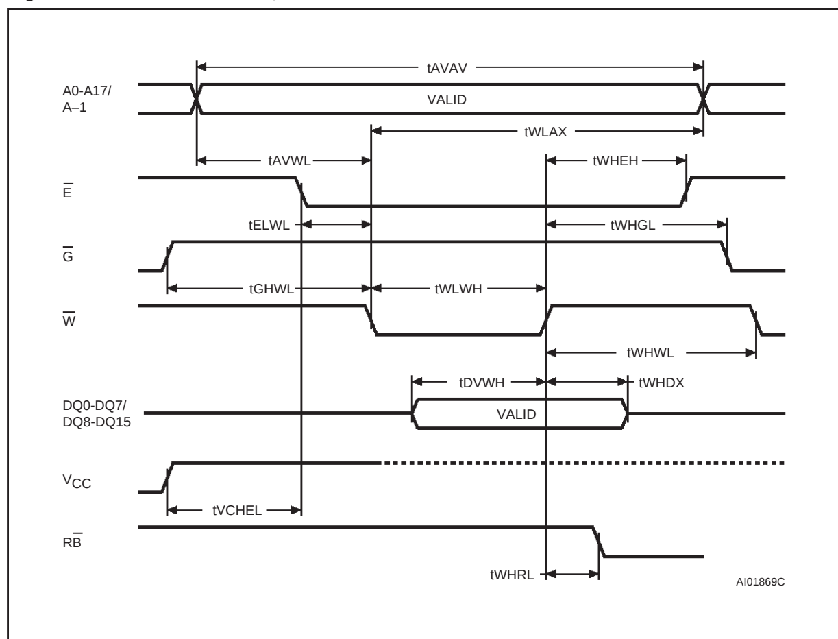
Note: Address are latched on the falling edge of \overline{W} . Data is latched on the rising edge of \overline{W} .
