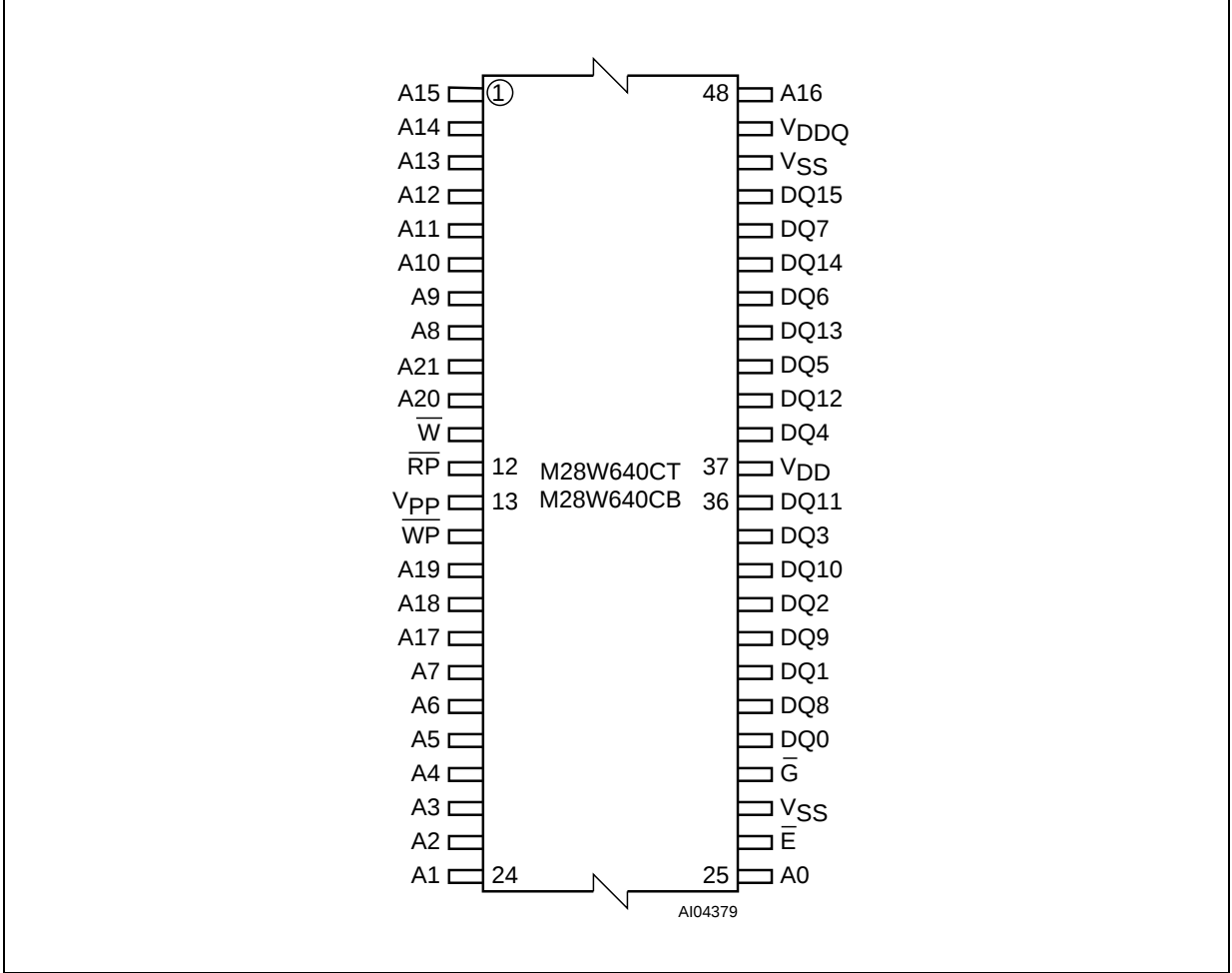
Figure 3. TSOP Connections
