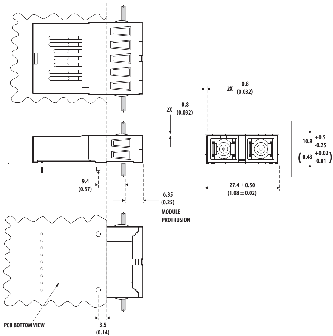
Figure 9. Suggested Module Positioning and Panel Cut-out for HFBR-5208EMZ
