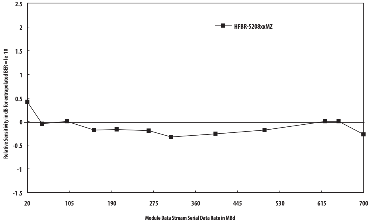
Figure 3. Relative Input Optical Power as a function of data rate normalized to center of Baud interval at 622 MBd. Test Conditions +25°C, 5.25 V, PRBS 2 23 -1, optical \tau_p/\tau_f = 0.9 ns with 3 m of MMF or SMF.
