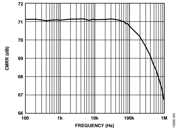
Figure 37. CMRR vs. Frequency, V_{DD} = 1.8 V, V_{IO} = 3.3 V, V_{REF} = 5 V, 25°C
