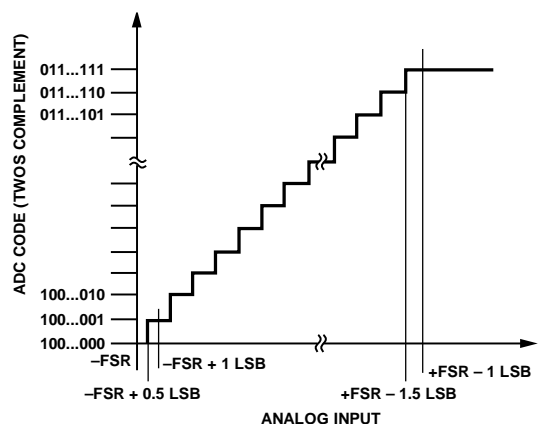
Figure 31. ADC Ideal Transfer Function (FSR Is Full-Scale Range)
