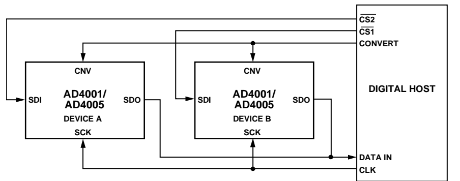
Figure 60. \overline{CS} Mode, 4-Wire Without Busy Indicator Connection Diagram
