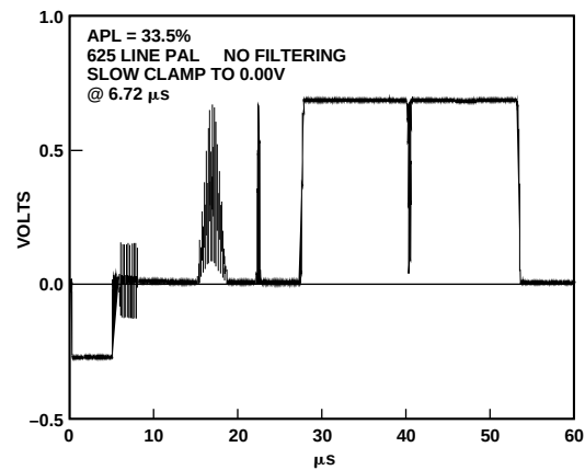
Figure 9. Modulated Pulse and Bar, PAL
