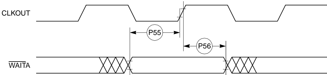
Figure 29. PCMCIA \overline{WAIT} Signals Detection Timing
