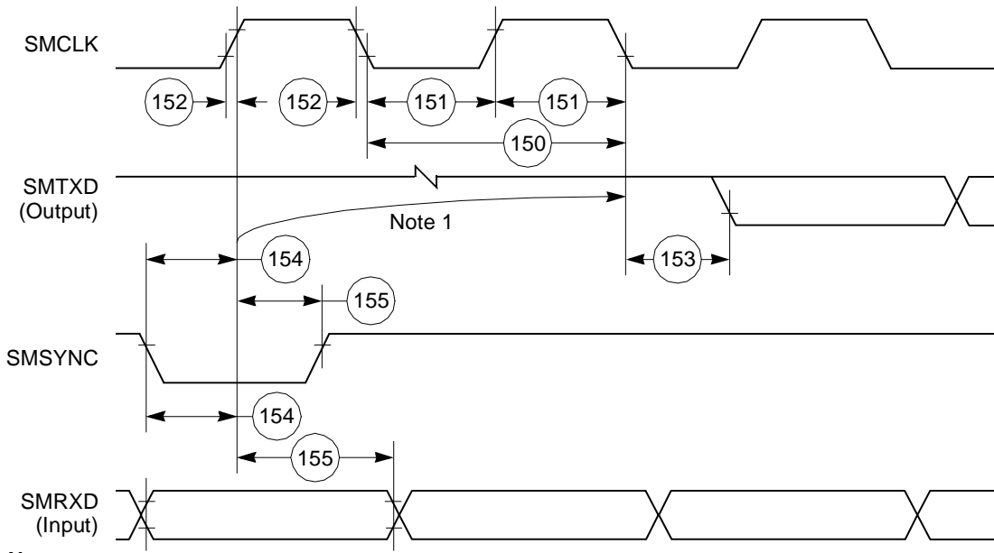
Figure 59. SMC Transparent Timing Diagram
