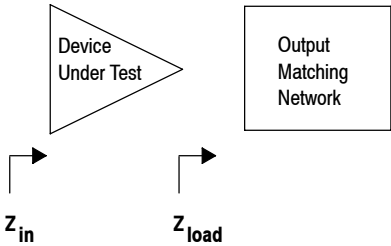
Figure 11. Series Equivalent Input and Load Impedance — 900 MHz
