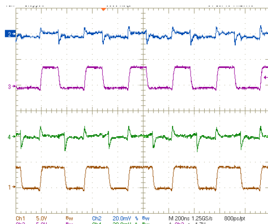
FIGURE 6. DCD OUTPUT RIPPLE ( V_{IN} = 4.2V , FULL LOADING @ VODCD1 AND VODCD2, TIME SCALE = 200ns) CH1: SW1 (5V/DIV), CH2: VODCD1 (20mV/DIV), CH3: SW2 (5V/DIV), CH4: VODCD2 (20mV/DIV)
