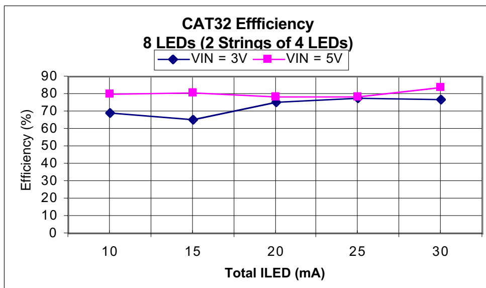
Figure 8. CAT32 Efficiency Driving 2 Parallel Strings of 4 LEDs in Series
