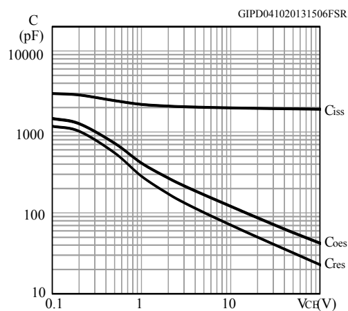
Figure 17. Capacitance variation
