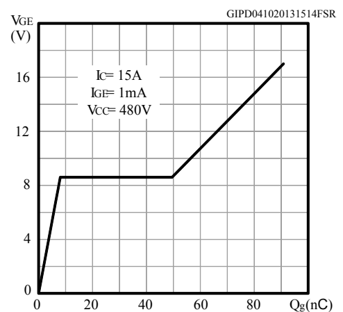
Figure 18. Gate charge vs gate-emitter voltage
