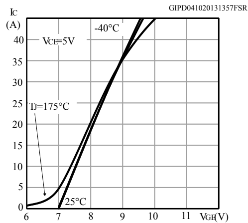
Figure 13. Transfer characteristics
