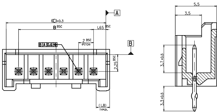
SECTION K-K'
