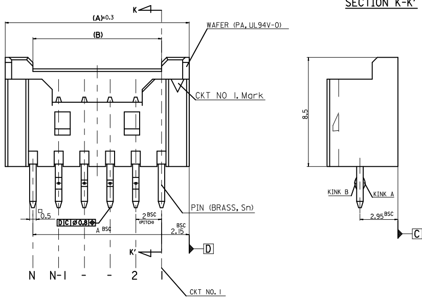
SECTION K-K'
