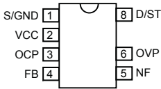
Pin-out Diagram
