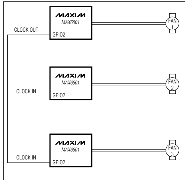
Figure 14. Synchronizing Fans
