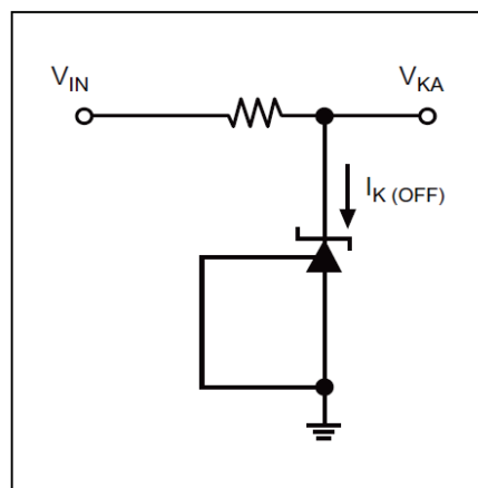
Fig. 27: Test Circuit for I_{K(OFF)}
