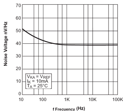
Fig. 8 Noise Voltage VS Frequency
