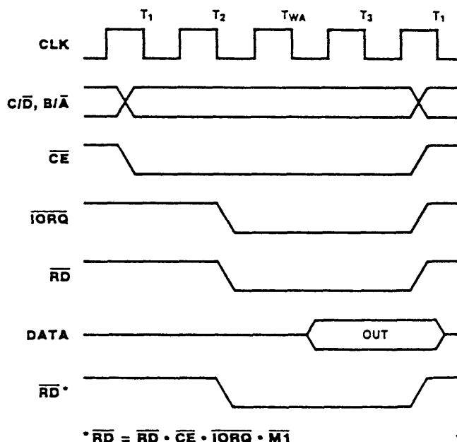
Figure 13. Read Cycle Timing
