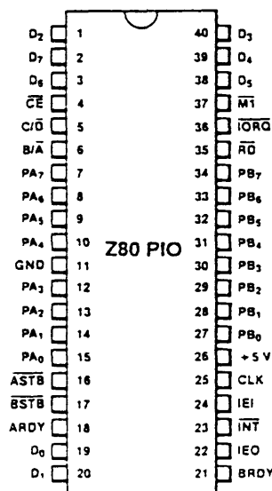
Figure 2a. 40-pin Dual-In-Line Package (DIP), Pin Assignments
