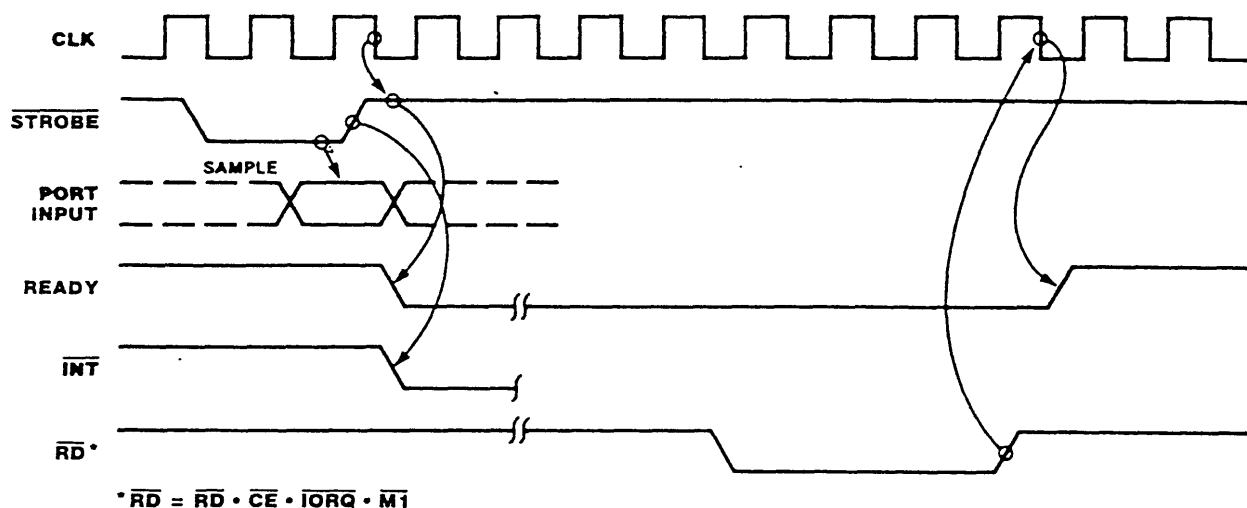
Figure 15. Mode 1 Input Timing
