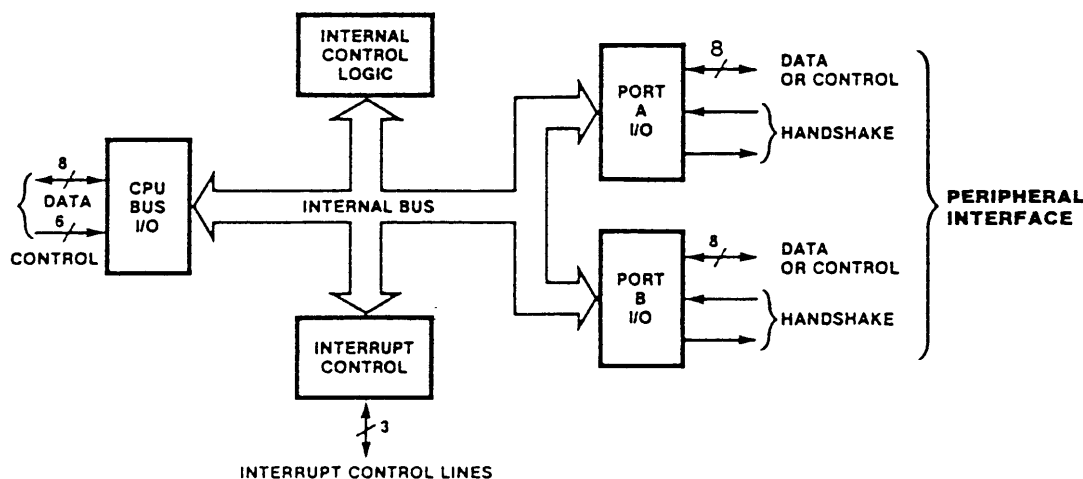
Figure 4. Block Diagram
