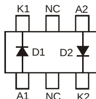
Internal Schematic
