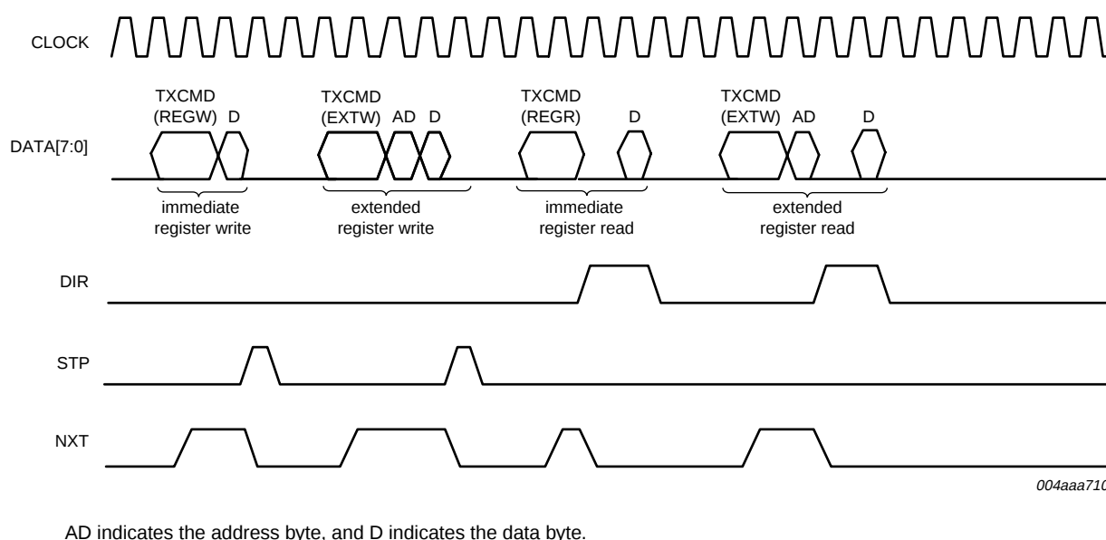
Fig 8. Example of register write, register read, extended register write and extended register read
