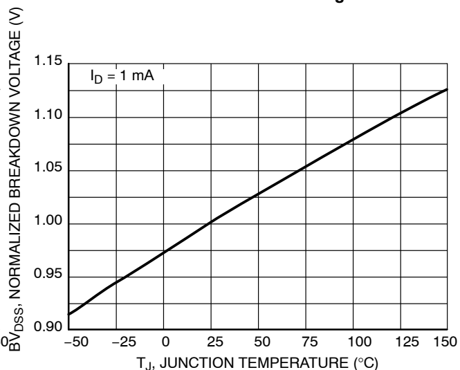
Figure 6. BV_{DSS} Variation with Temperature
