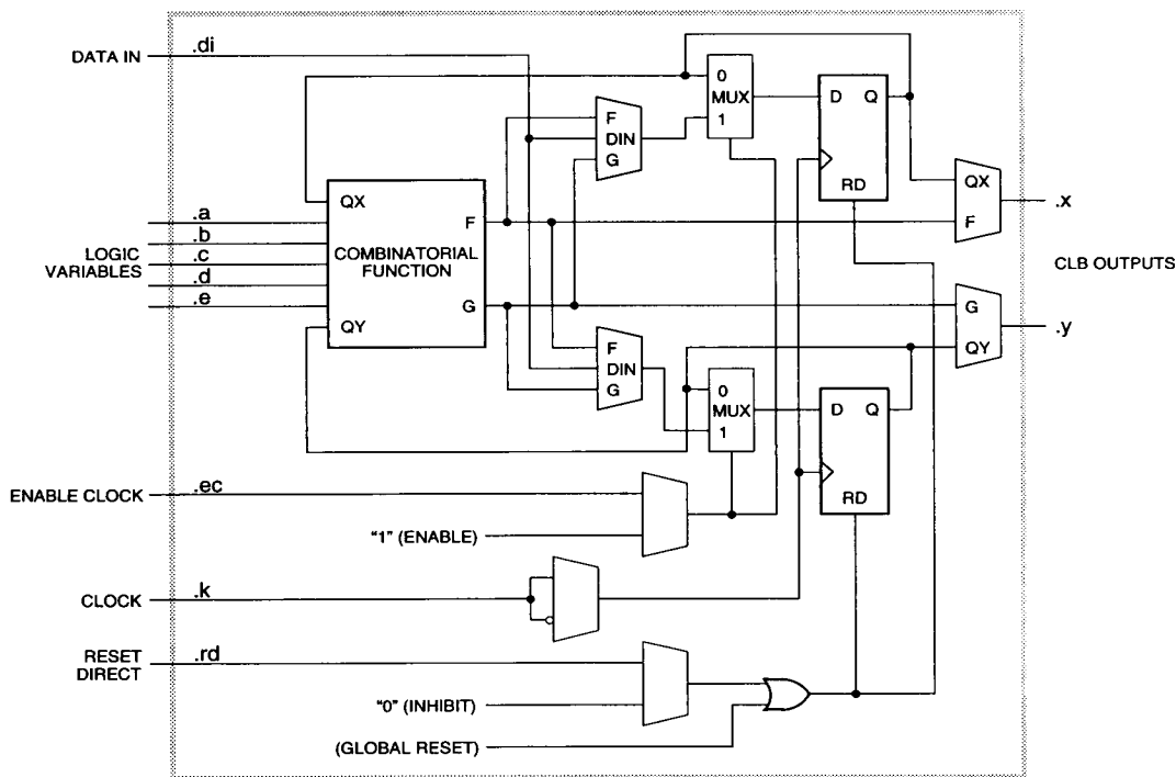
Figure 4. Configurable Logic Block. Each CLB includes a combinational logic, two flip-flops and a program memory controlled multiplexer selection of function.
