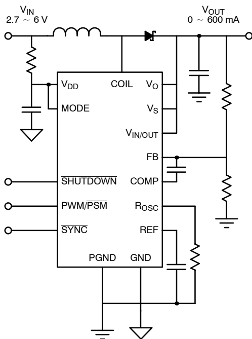
Boost Configuration
