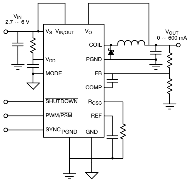
Buck Configuration
