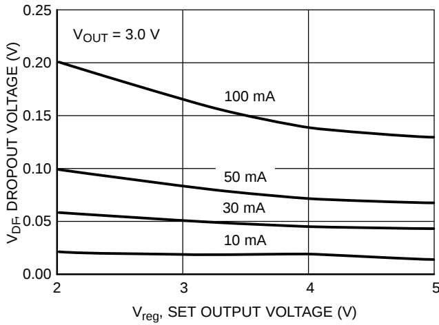
Figure 27. Dropout Voltage vs. Set Output Voltage
