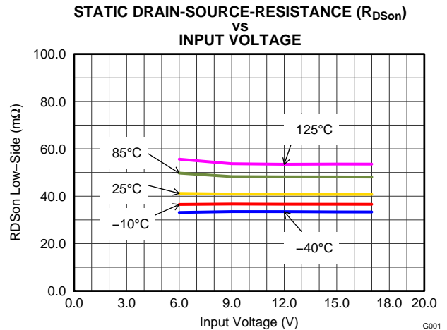
Figure 24. Low-Side Switch Resistance
