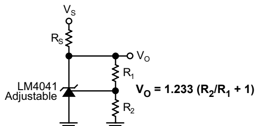
Figure 2. LM4041 Adjustable Shunt Regulator Application
