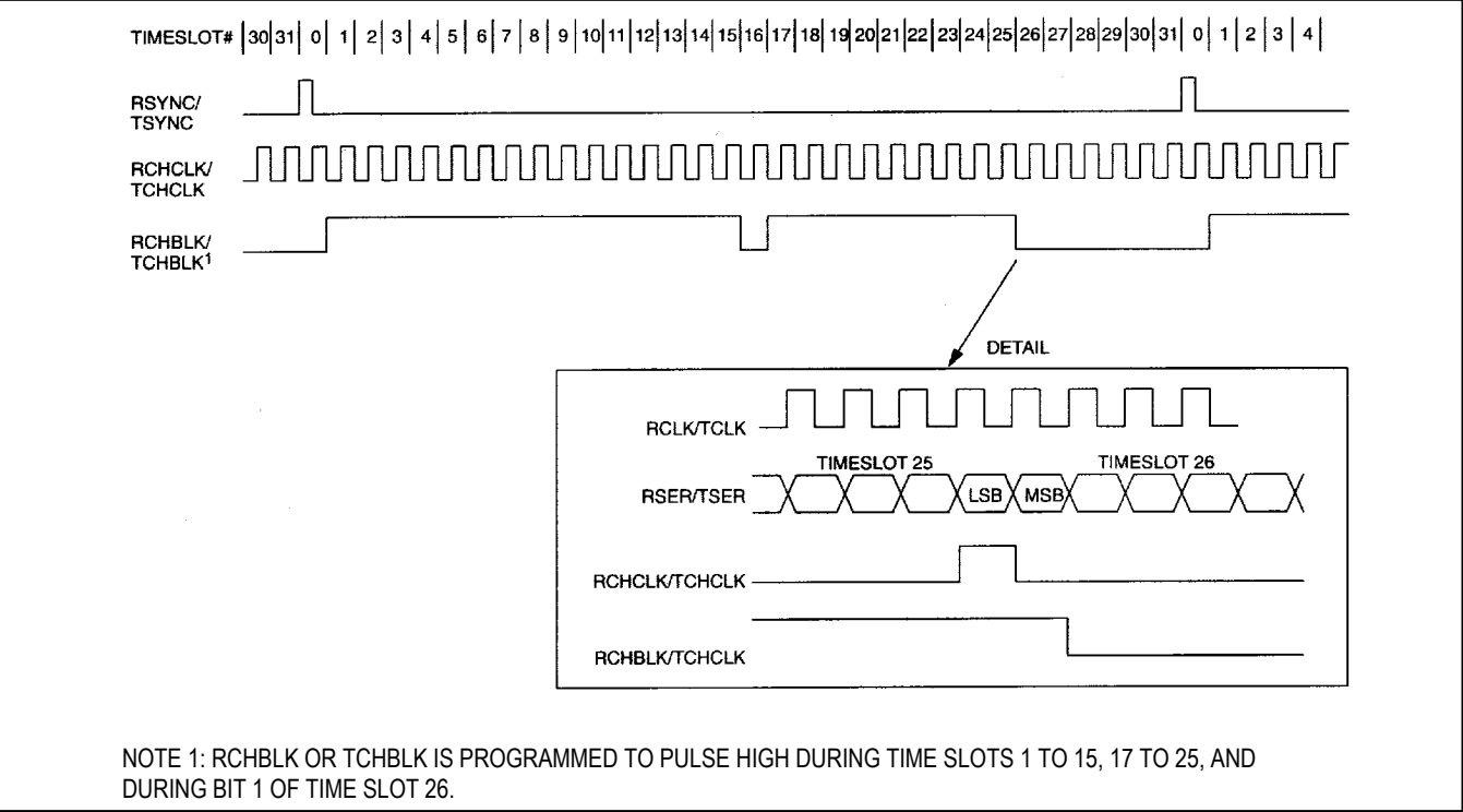
Figure 14-7. G.802 Timing
