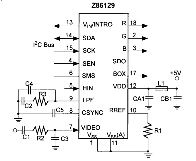
Figure 40. Z86129 Application Circuit with I 2 C
