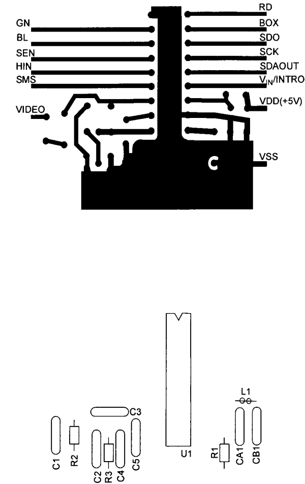
Figure 41. Z86129 Application Circuit with I 2 C
