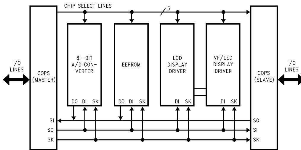
FIGURE 29. MICROWIRE/PLUS Application
