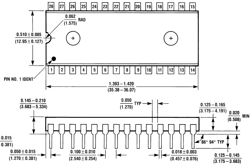
Molded Dual-In-Line Package (N) Order Number COP8SGx728Nx NS Package Number N28A
