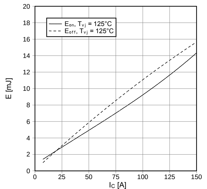
Schaltverluste IGBT-Wechselr. (typisch) switching losses IGBT-inverter (typical) E_{on} = f(I_C) , E_{off} = f(I_C) V_{GE} = \pm 15 \text{ V} , R_{Gon} = 11 \Omega , R_{Goff} = 11 \Omega , V_{CE} = 600 \text{ V}
