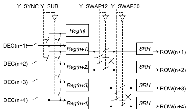
Figure 10. Row Structure
