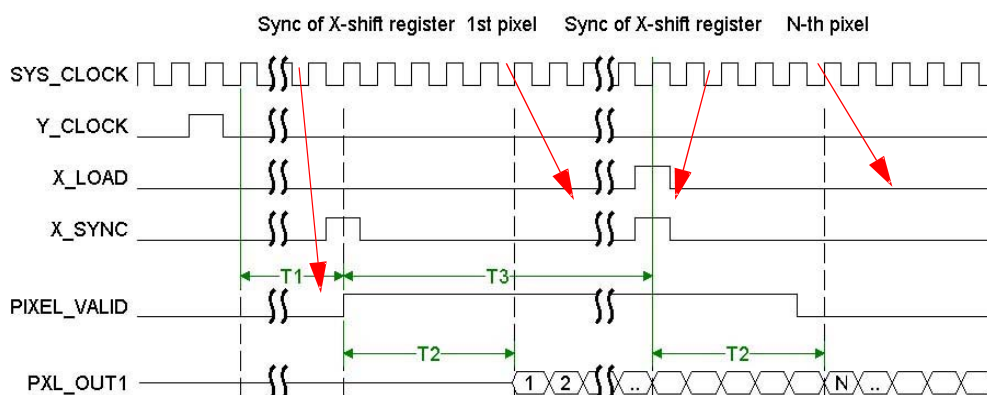
Figure 24. Pixel Output
