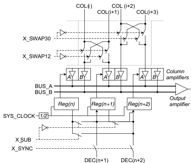
Figure 9. Column Structure
