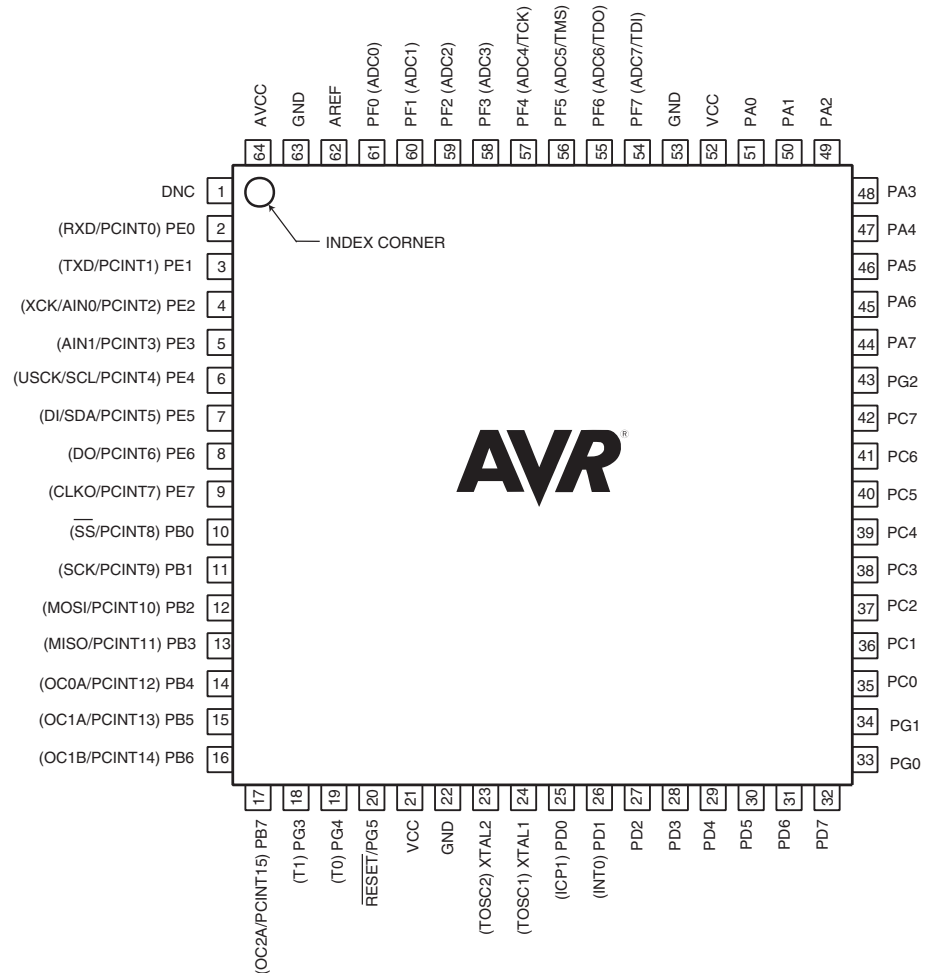
Figure 1-1. Pinout ATmega165P
