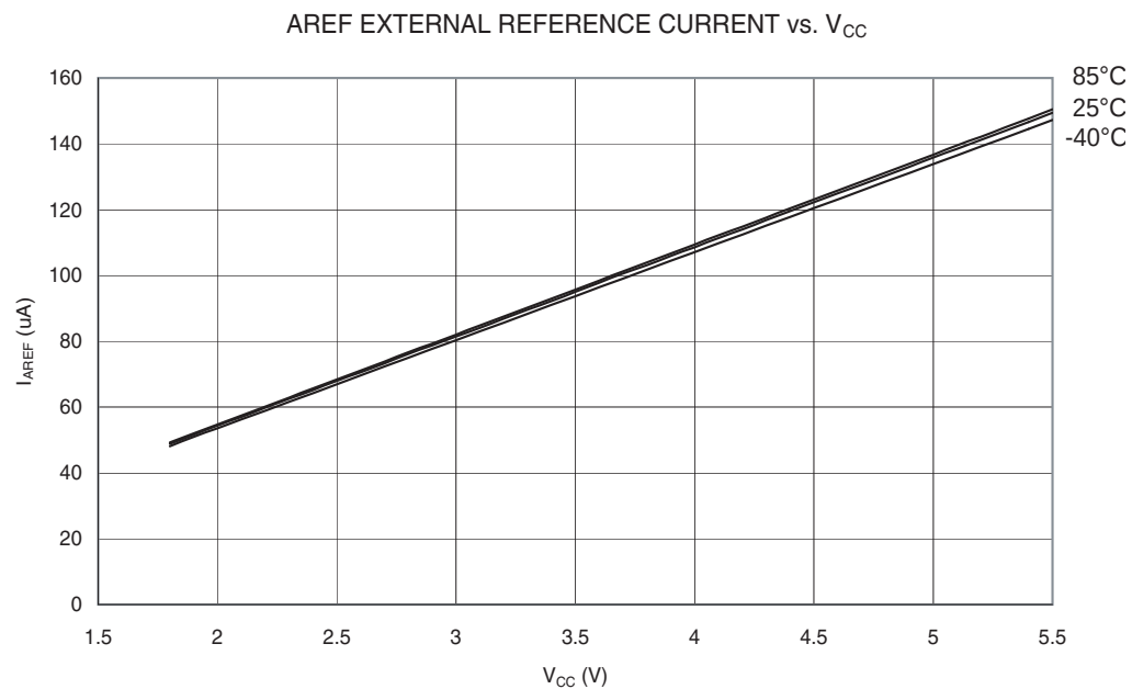
Figure 27-60. AREF External Reference Current vs. V_{CC}
