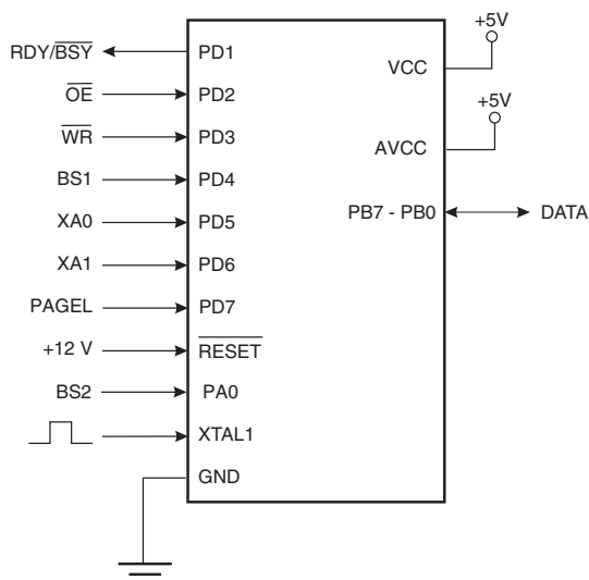
Figure 25-1. Parallel Programming
