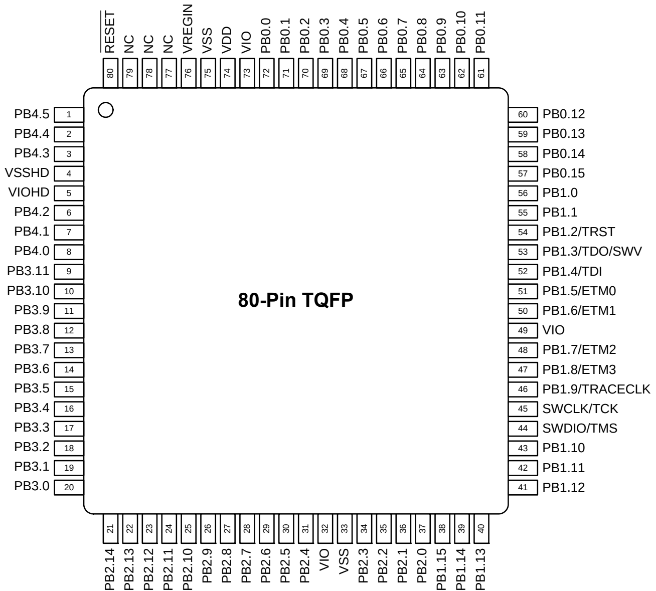
Figure 6.1. SiM3C1x7-GQ Pinout
