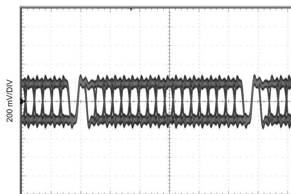
Figure 23. Serial Output Quad Mode, 85 MHz, VSEL = L, No Pre-Emphasis
