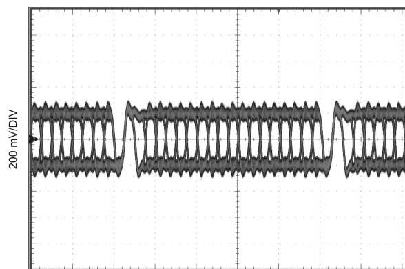
Figure 25. Serial Output Dual Mode, 50 MHz, VSEL = L, No Pre-Emphasis
