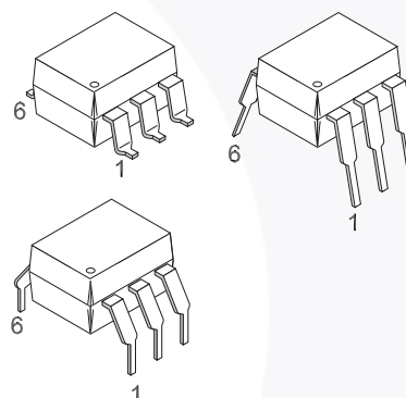
Figure 1. Package Outlines
