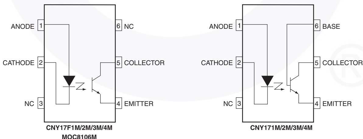
Figure 2. Schematics
