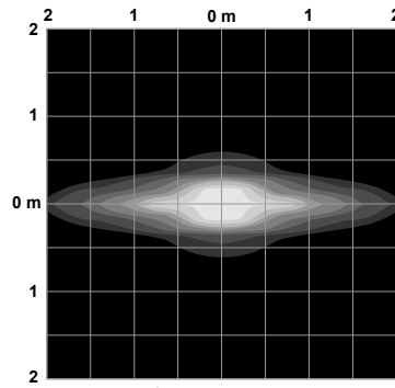
Isolux Pattern
