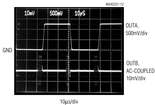
ANALOG CROSSTALK
