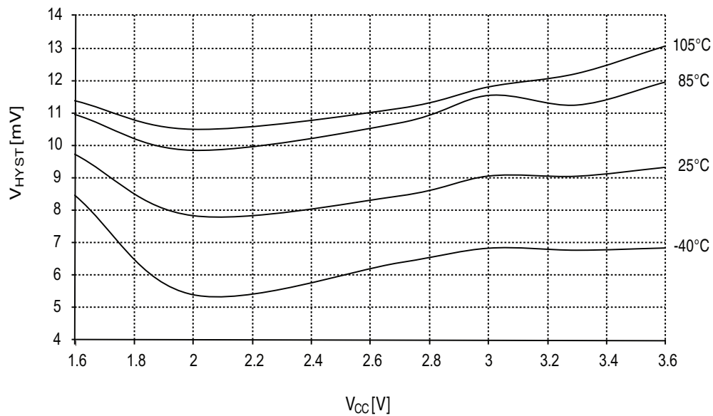
Figure 33-48. Analog comparator hysteresis vs. V_{CC} .
