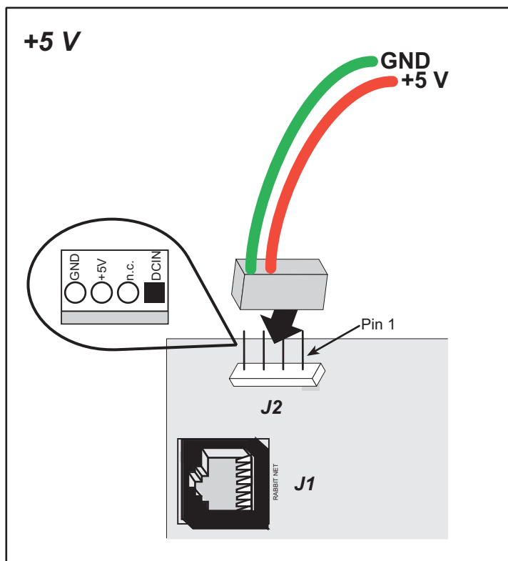
Figure 19. Power-Supply Connections
