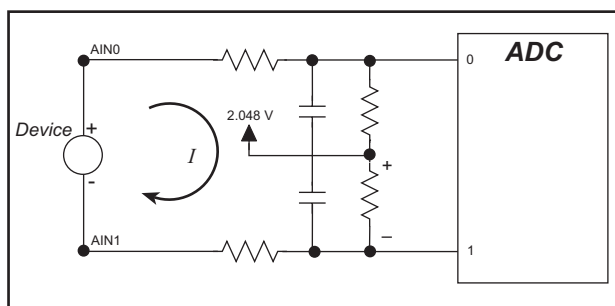
Figure 22. Current Flow from Ungrounded or Floating Source
