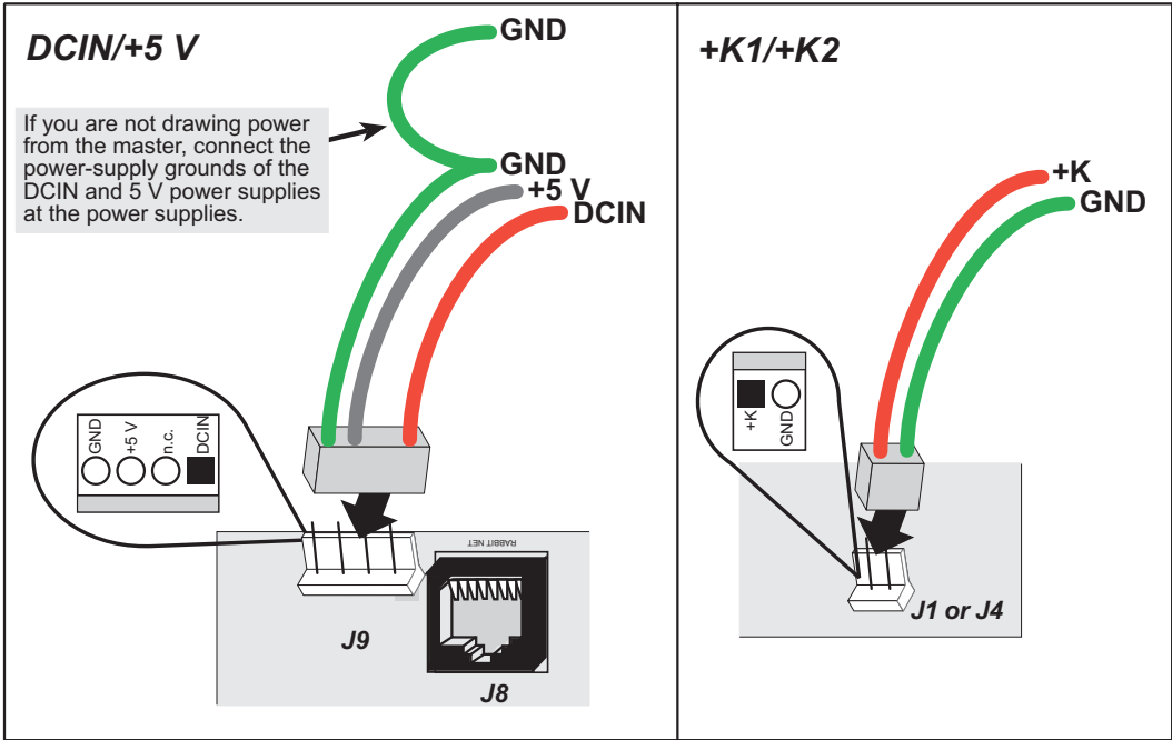
Figure 5. Power-Supply Connections
