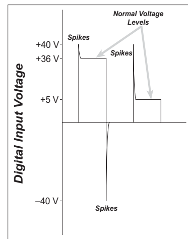
Figure 10. RN1100 Digital Input Protected Range
