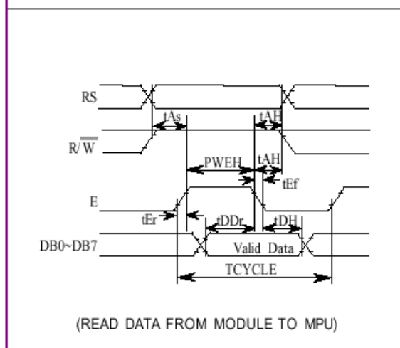
FIG 2. READ OPERATION
