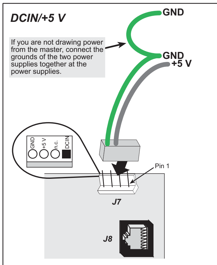
Figure 36. Power-Supply Connections
