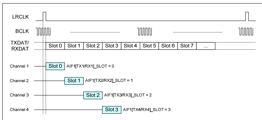
Figure 49 DSP Mode A Example
