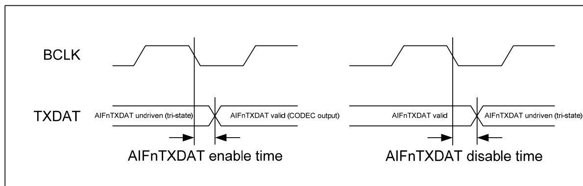
Figure 8 Audio Interface Timing - TDM Mode
