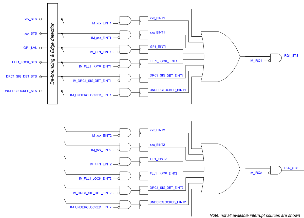
Figure 67 Interrupt Controller
