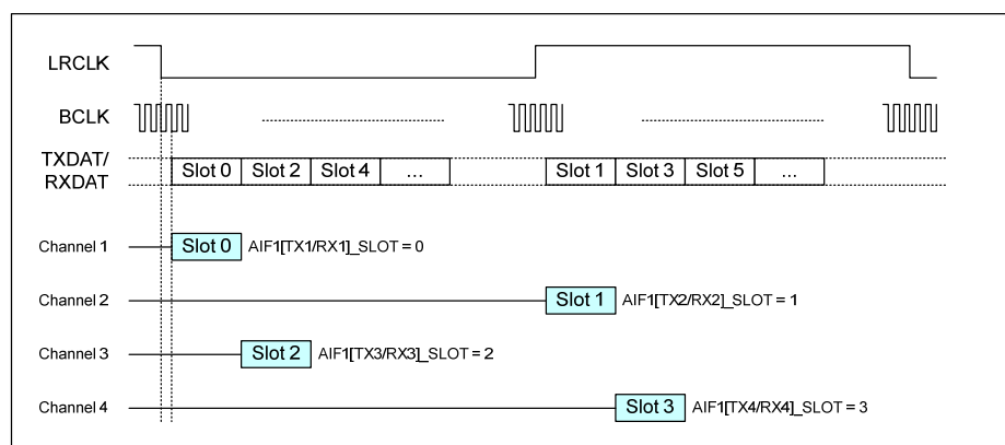
Figure 51 I2S Example
