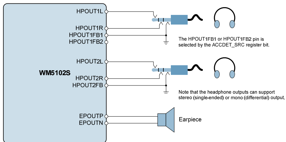
Figure 86 Headphone and Earpiece Connection
