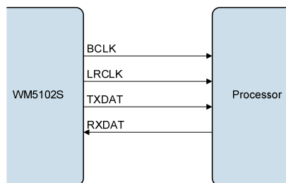
Figure 43 Master Mode
