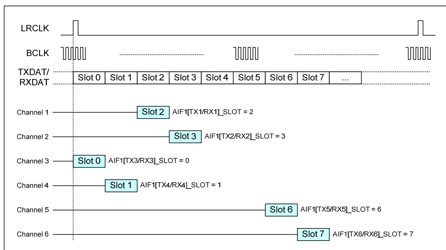
Figure 50 DSP Mode B Example
