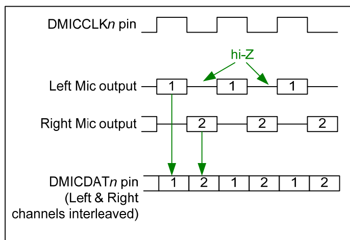
Figure 21 Digital Microphone Interface Timing
