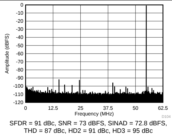
Figure 97. FFT for 70-MHz Input Signal (Dither Off)
