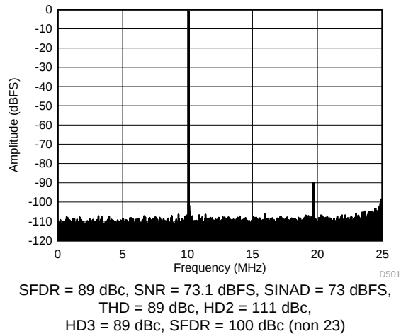
Figure 32. FFT for 10-MHz Input Signal (Dither On)
