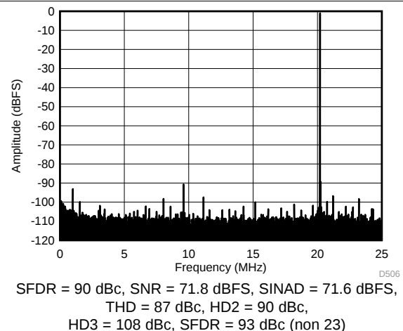
Figure 37. FFT for 170-MHz Input Signal (Dither Off)
