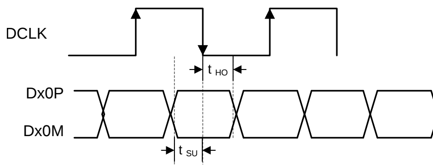
Figure 135. Setup and Hold Time
