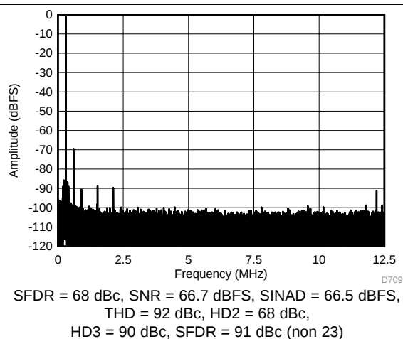
Figure 9. FFT for 450-MHz Input Signal (Dither On)
