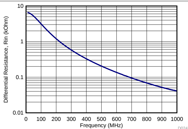
Figure 185. Differential Input Resistance, R_{IN}
