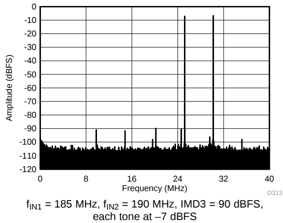
Figure 75. FFT FOR Two-Tone Input Signal ( -7\text{ dBFS} at 185 MHz and 190 MHz)
