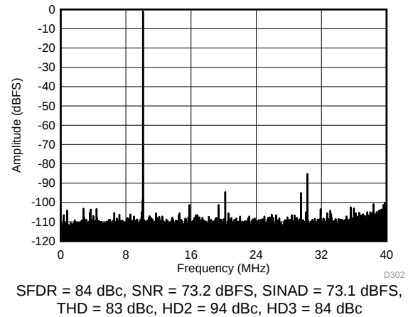
Figure 64. FFT for 10-MHz Input Signal (Dither Off)
