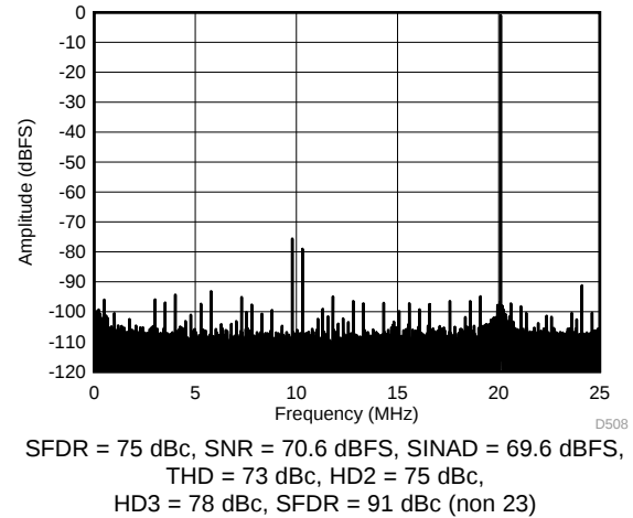
Figure 39. FFT for 270-MHz Input Signal (Dither Off)
