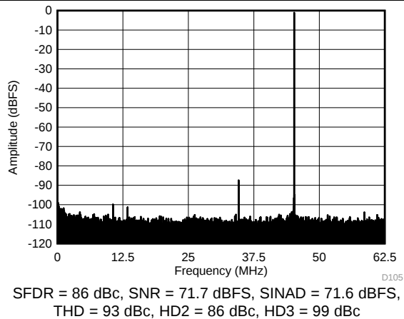
Figure 98. FFT for 170-MHz Input Signal (Dither On)
