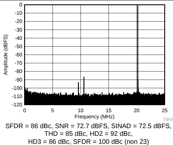
Figure 34. FFT for 70-MHz Input Signal (Dither On)
