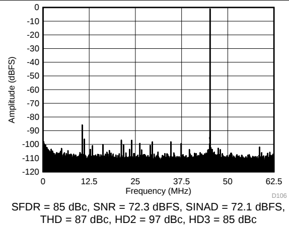
Figure 99. FFT for 170-MHz Input Signal (Dither Off)
