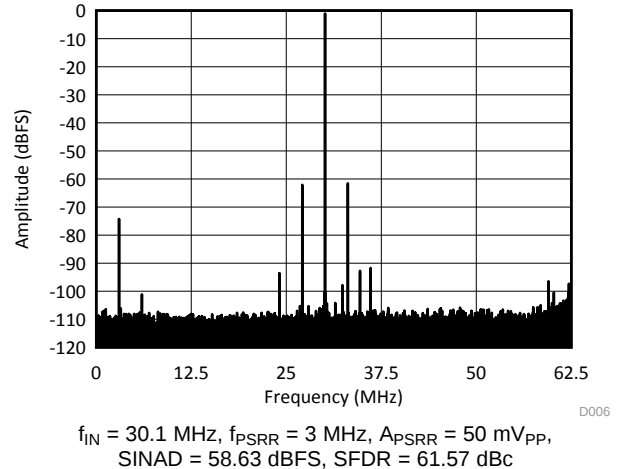
Figure 126. Power-Supply Rejection Ratio Spectrum
