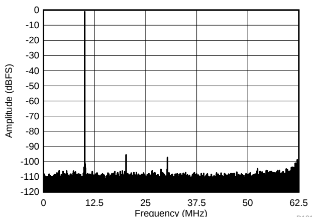
Spectrum at 10-MHz IF (SFDR = 95 dBc, SNR = 72.7 dBFS, SINAD = 72.6 dBFS, THD = 100 dBc, HD2 = 95 dBc, HD3 = 96 dBc)
