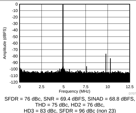
Figure 7. FFT for 270-MHz Input Signal (Dither On)
