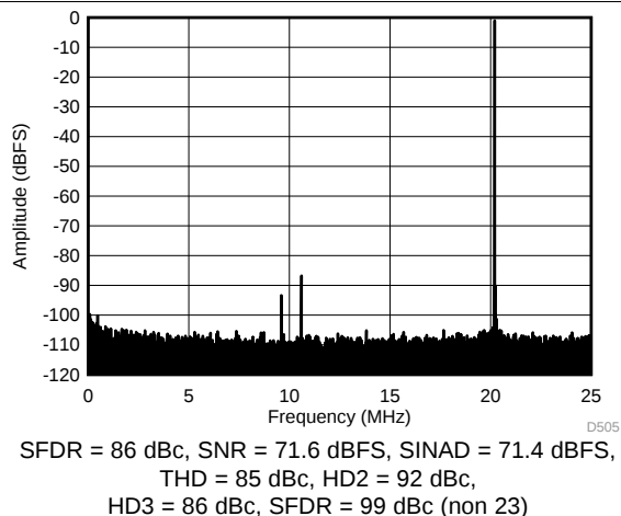
Figure 36. FFT for 170-MHz Input Signal (Dither On)
