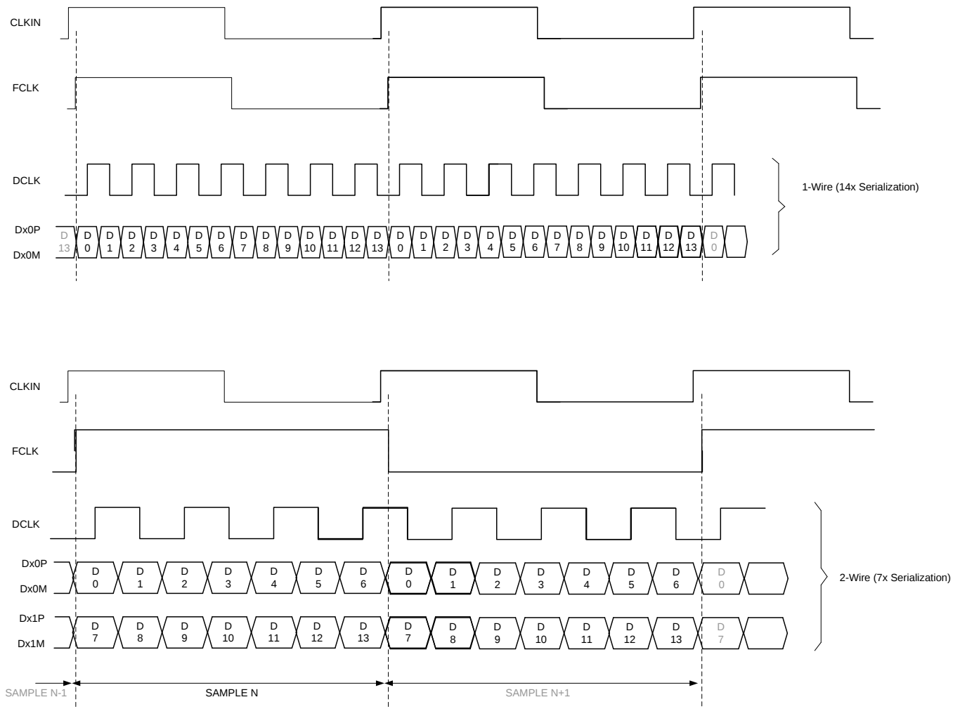
Figure 134. Output Timing Diagram
