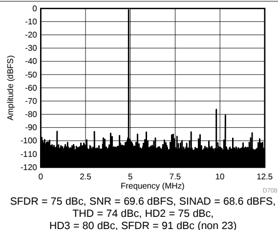
Figure 8. FFT for 270-MHz Input Signal (Dither Off)
