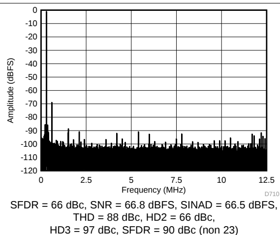
Figure 10. FFT for 450-MHz Input Signal (Dither Off)
