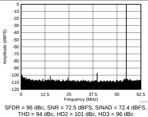
Figure 96. FFT for 70-MHz Input Signal (Dither On)
