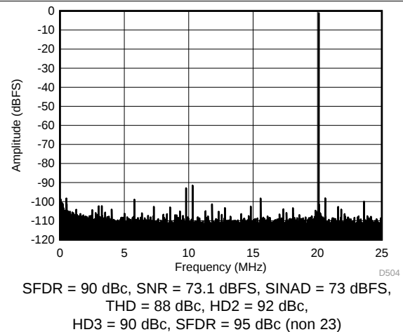
Figure 35. FFT for 70-MHz Input Signal (Dither Off)
