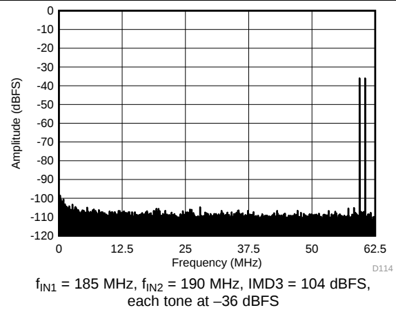
Figure 107. FFT for Two-Tone Input Signal ( -36\text{ dBFS} at 185 MHz and 190 MHz)
