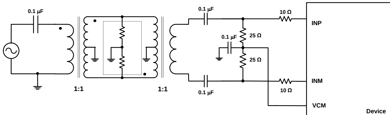
Figure 191. Driving Circuit for High Input Frequencies ( f_{IN} > 230 MHz)
