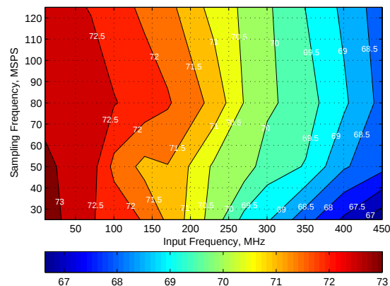
Figure 132. Signal-to-Noise Ratio (SNR)
