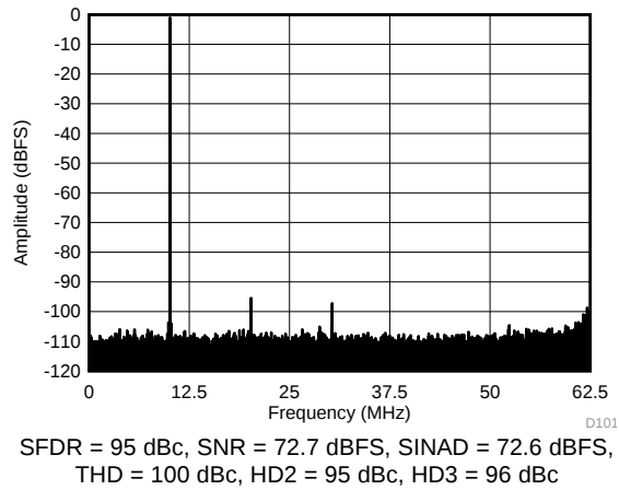
Figure 94. FFT for 10-MHz Input Signal (Chopper On, Dither On)
