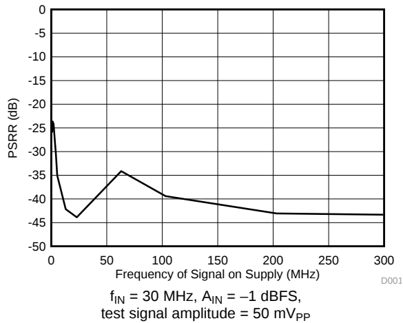
Figure 125. Power-Supply Rejection Ratio vs Test Signal Frequency
