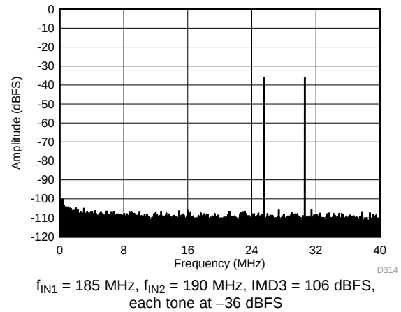
Figure 76. FFT FOR Two-Tone Input Signal ( -36\text{ dBFS} at 185 MHz and 190 MHz)
