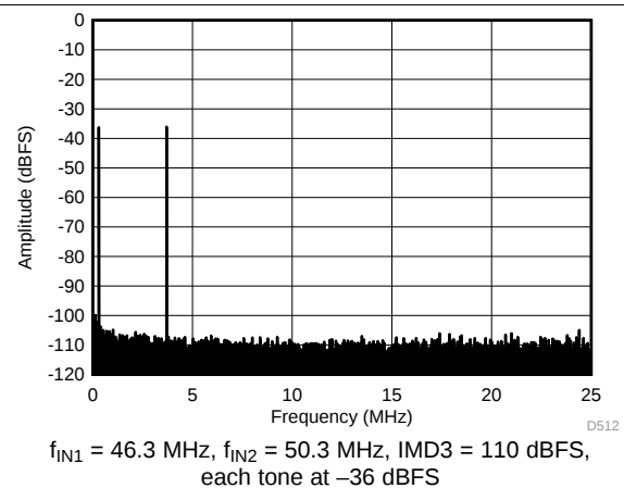
Figure 43. FFT for Two-Tone Input Signal ( -36\text{ dBFS} at 46 MHz and 50 MHz)
