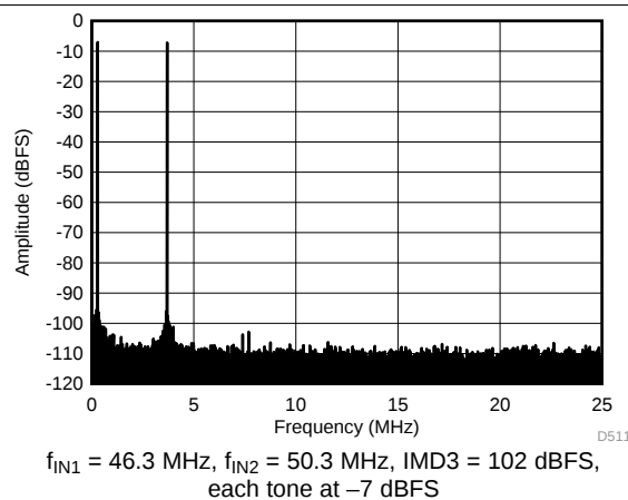
Figure 42. FFT for Two-Tone Input Signal ( -7\text{ dBFS} at 46 MHz and 50 MHz)
