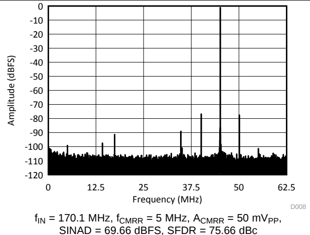
Figure 128. Common-Mode Rejection Ratio Spectrum
