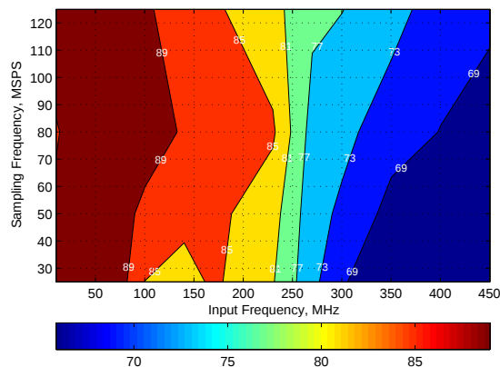
Figure 131. Spurious-Free Dynamic Range (SFDR)
