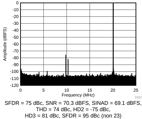
Figure 38. FFT for 270-MHz Input Signal (Dither On)
