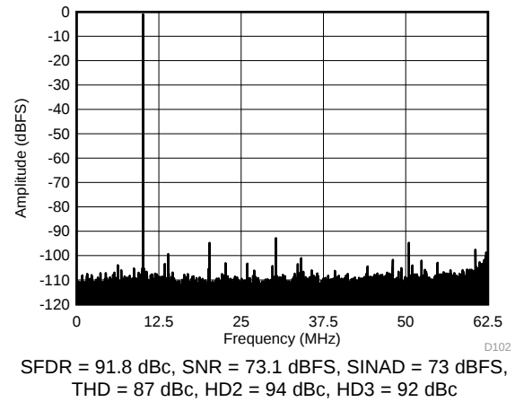
Figure 95. FFT for 10-MHz Input Signal (Chopper On, Dither Off)
