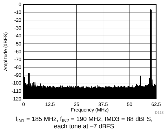
Figure 106. FFT for Two-Tone Input Signal ( -7\text{ dBFS} at 185 MHz and 190 MHz)
