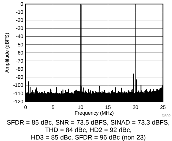
Figure 33. FFT for 10-MHz Input Signal (Dither Off)
