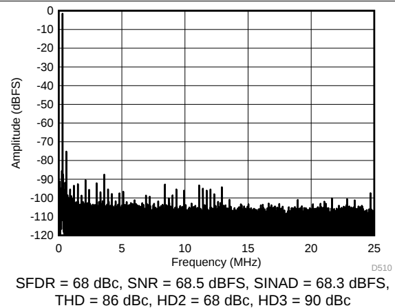
Figure 41. FFT for 450-MHz Input Signal (Dither Off)
