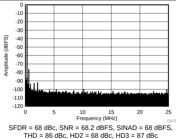
Figure 40. FFT for 450-MHz Input Signal (Dither On)
