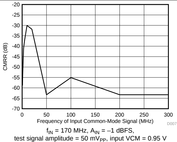
Figure 127. Common-Mode Rejection Ratio vs Test Signal Frequency
