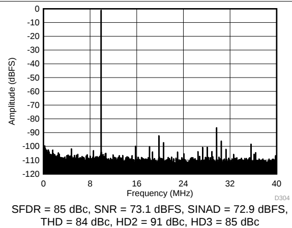
Figure 66. FFT for 70-MHz Input Signal (Dither Off)
