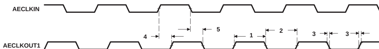
Figure 4–15. AECLKOUT1 Timing for the EMIFA Module
