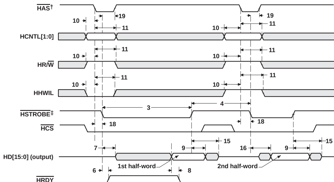
Figure 4-39. HPI16 Read Timing ( \overline{\text{HAS}} Used)
