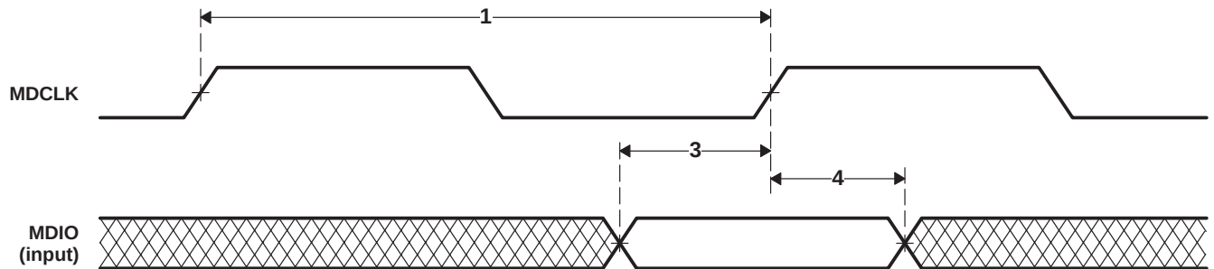
Figure 4–67. MDIO Input Timing
