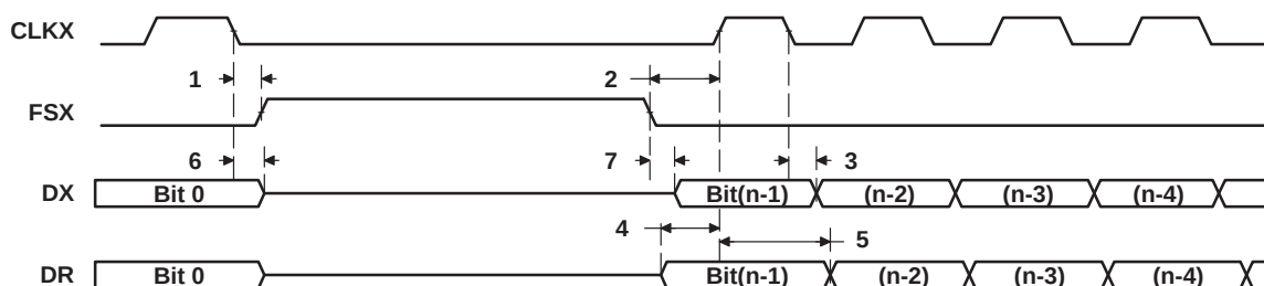
Figure 4–54. McBSP Timing as SPI Master or Slave: CLKSTP = 11b, CLKXP = 0
