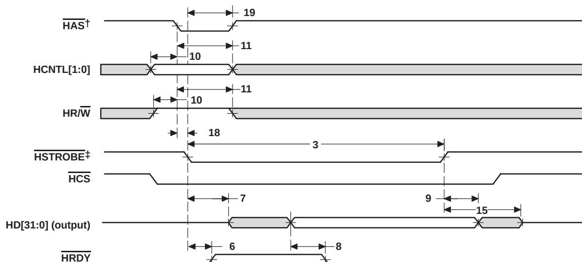
Figure 4-43. HPI32 Read Timing ( \overline{\text{HAS}} Used)
