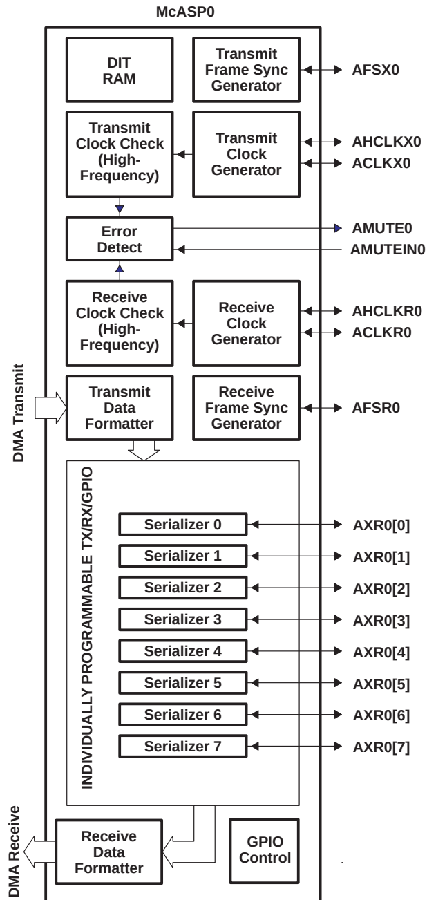
Figure 4–32. McASP0 Configuration
