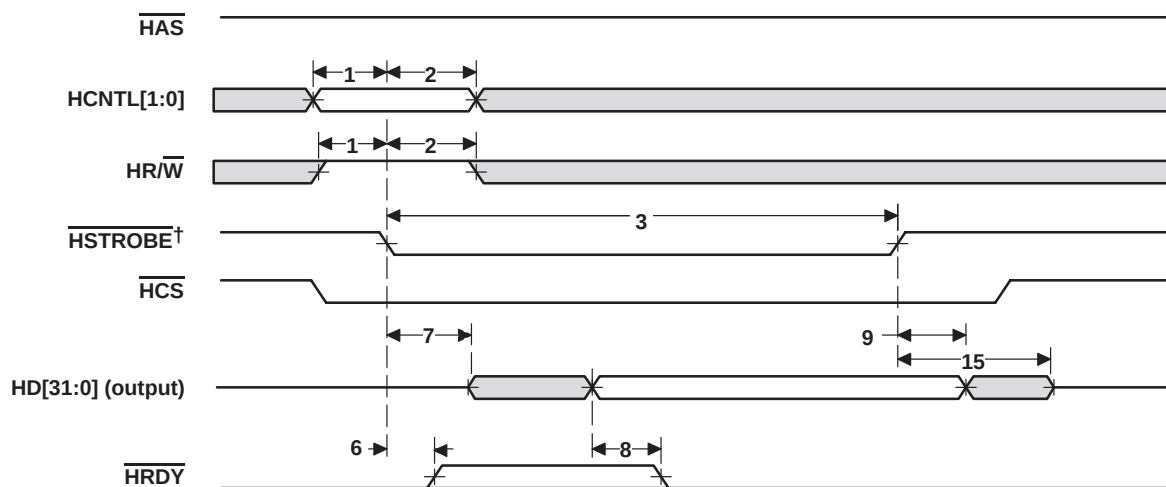
Figure 4-42. HPI32 Read Timing ( \overline{\text{HAS}} Not Used, Tied High)
