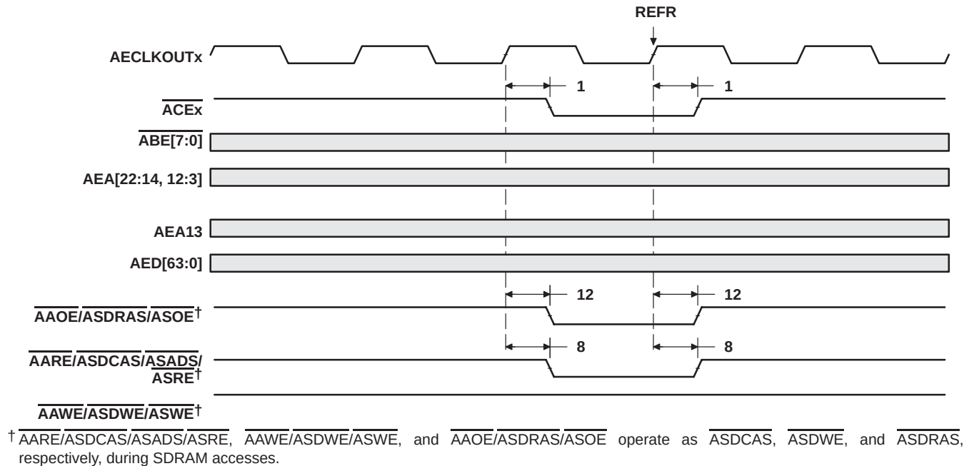
Figure 4-27. SDRAM REFR Command for EMIFA
