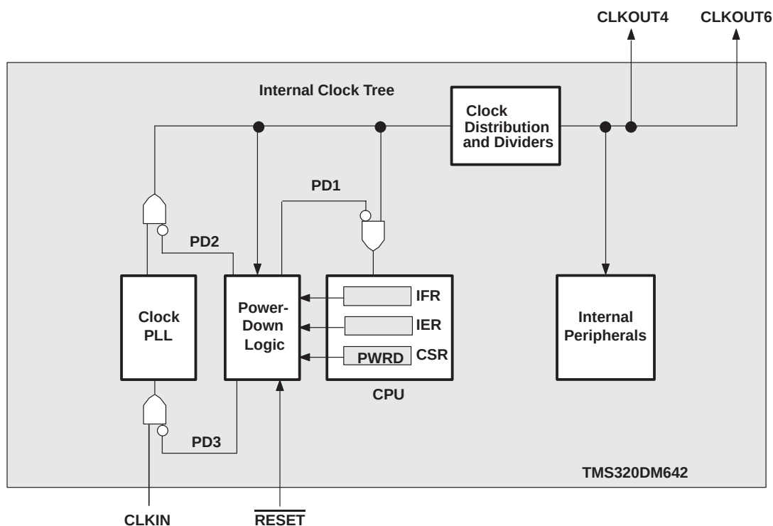
Figure 4–6. Power-Down Mode Logic†
