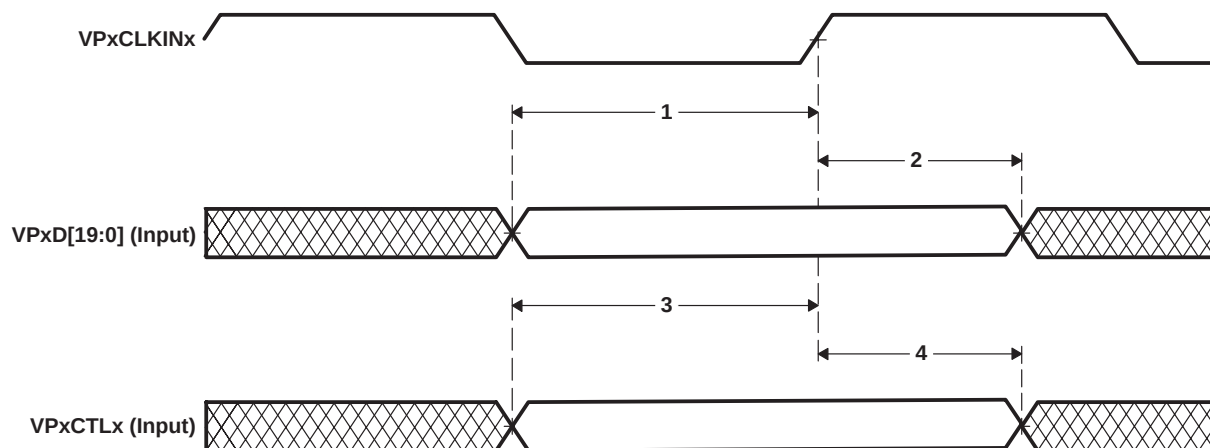
Figure 4–58. Video Port Capture Data and Control Input Timing
