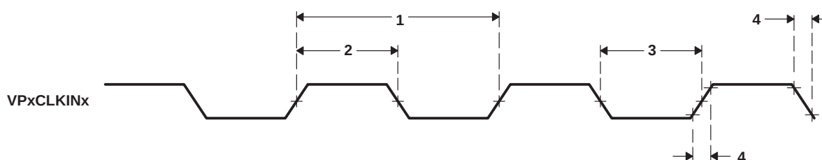
Figure 4–57. Video Port Capture VPxCLKINx Timing
