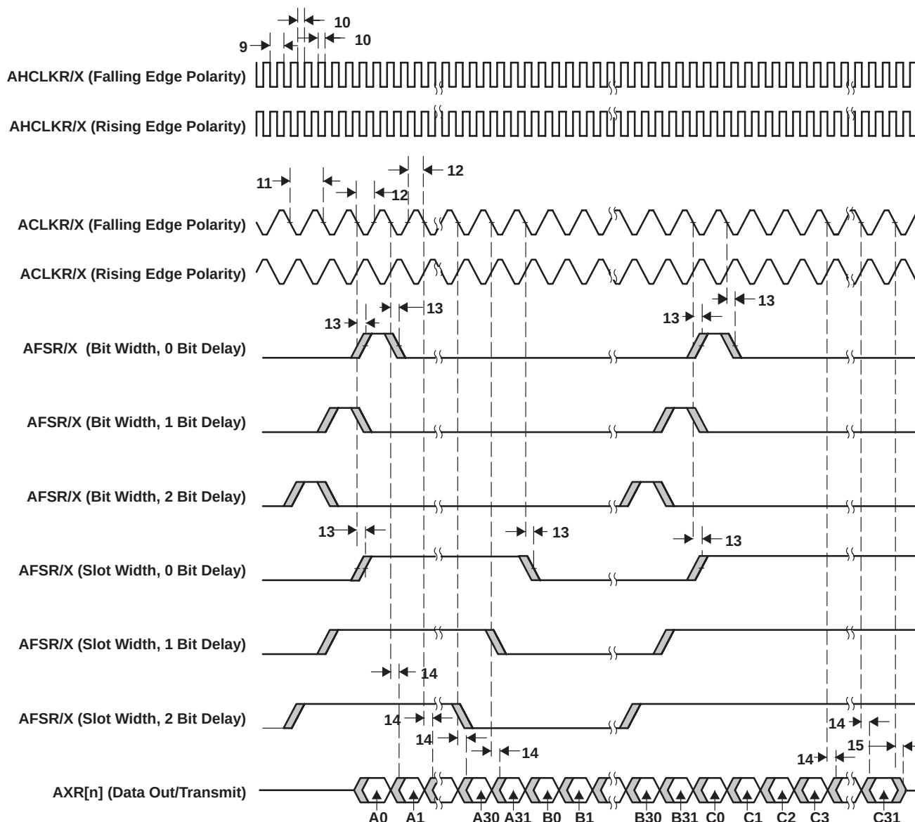
Figure 4-34. McASP Output Timings
