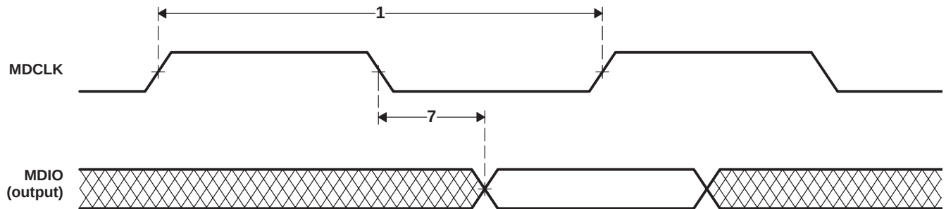
Figure 4–68. MDIO Output Timing
