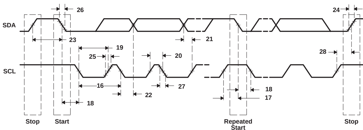
Figure 4–37. I2C Transmit Timings
