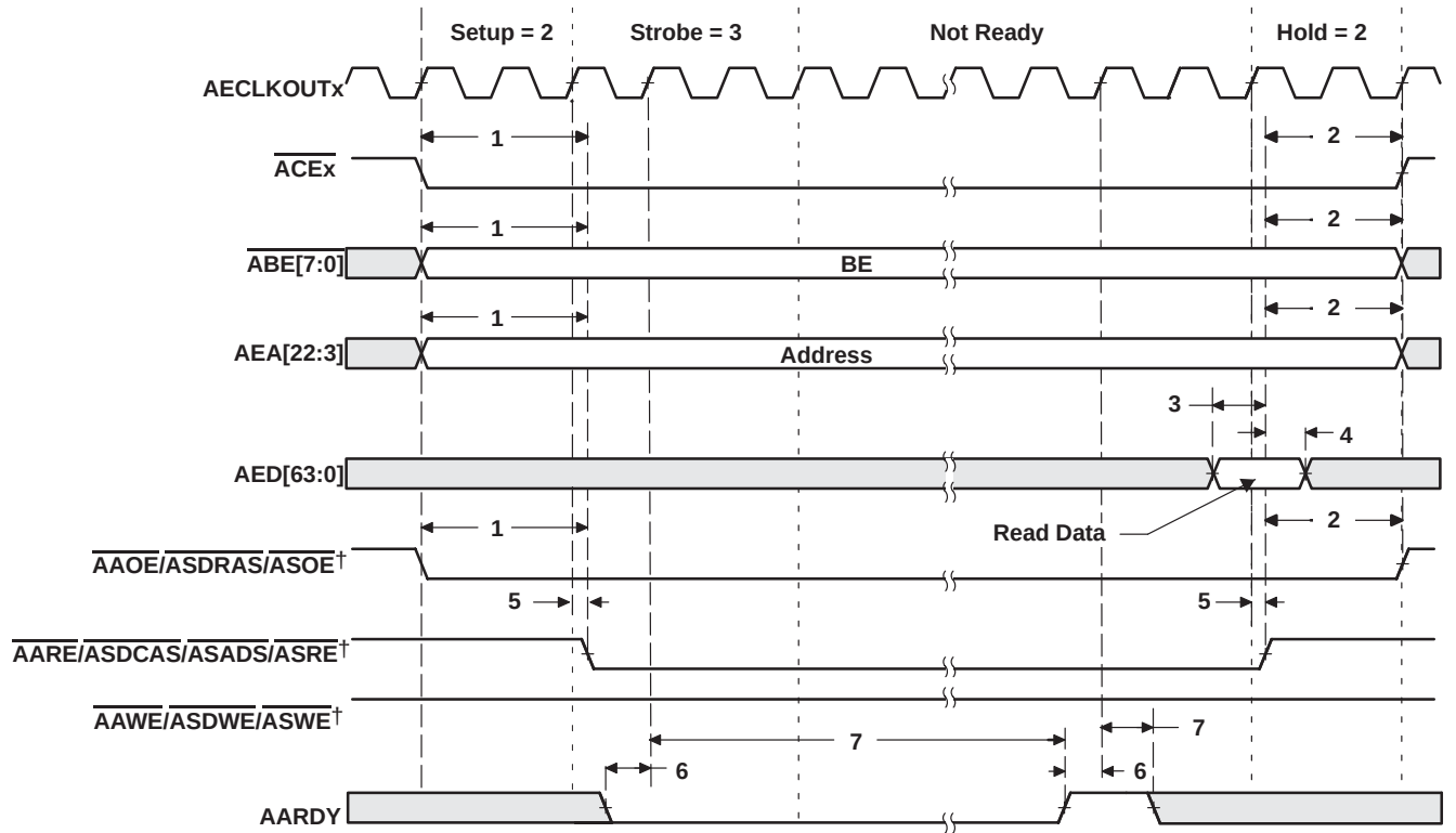
Figure 4–17. Asynchronous Memory Read Timing for EMIFA
