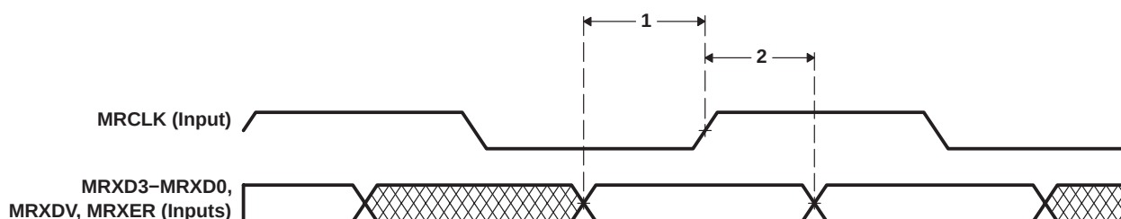
Figure 4-65. EMAC Receive Interface Timing
