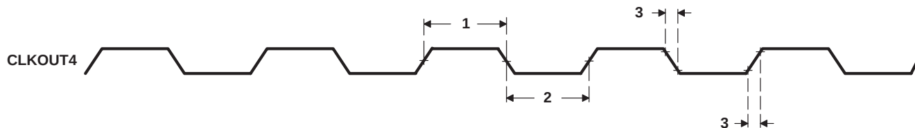
Figure 4-12. CLKOUT4 Timing
