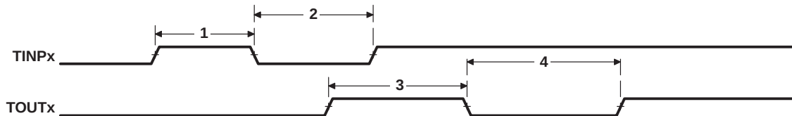
Figure 4–69. Timer Timing
