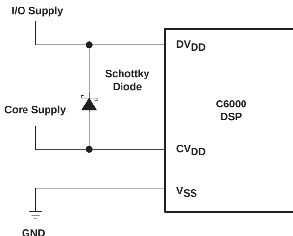
Figure 4–5. Schottky Diode Diagram
