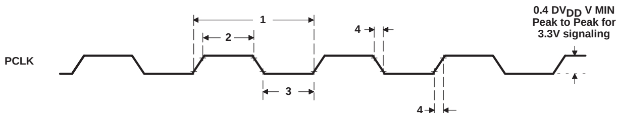
Figure 4-46. PCLK Timing
