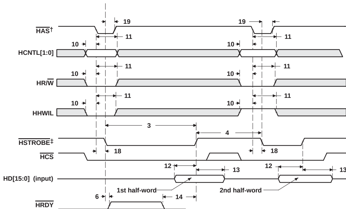
Figure 4-41. HPI16 Write Timing ( \overline{\text{HAS}} Used)
