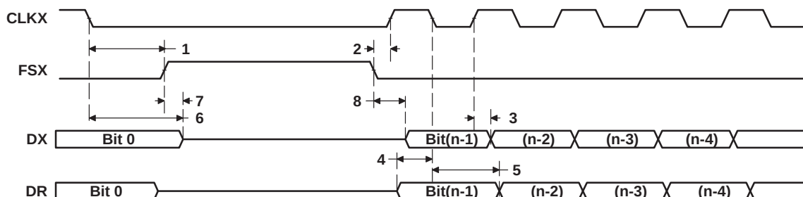
Figure 4–53. McBSP Timing as SPI Master or Slave: CLKSTP = 10b, CLKXP = 0
