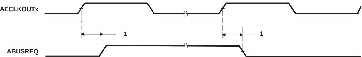
Figure 4–31. BUSREQ Timing for EMIFA
