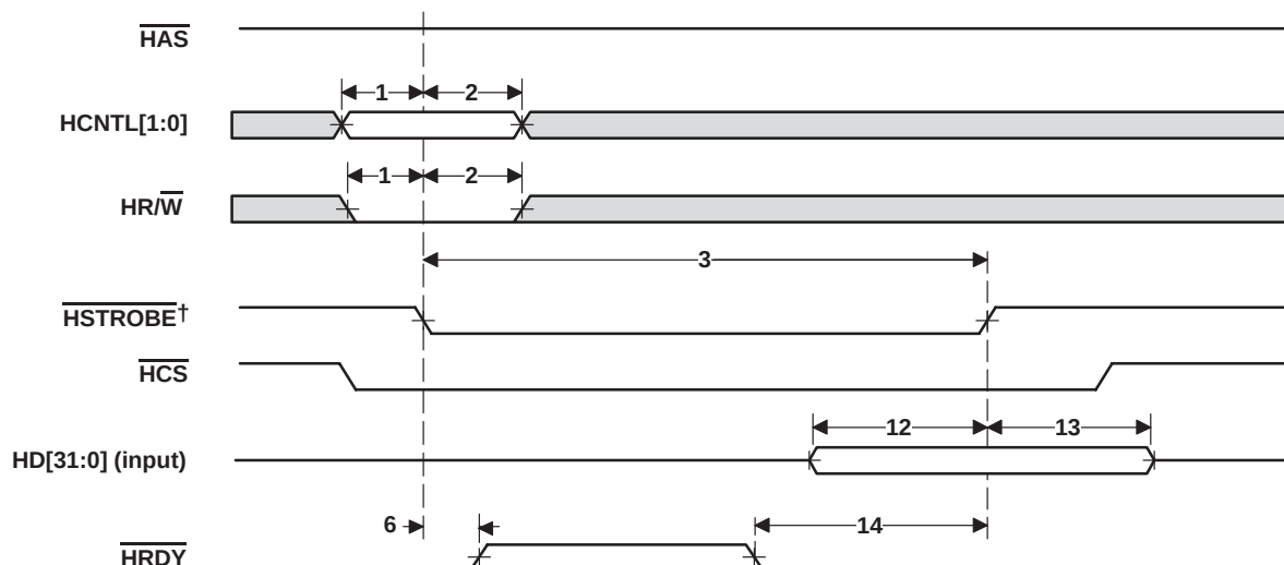
Figure 4-44. HPI32 Write Timing ( \overline{\text{HAS}} Not Used, Tied High)
