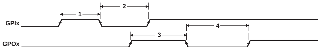
Figure 4–72. GPIO Port Timing
