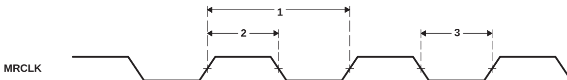
Figure 4–63. MRCLK Timing (EMAC – Receive)
