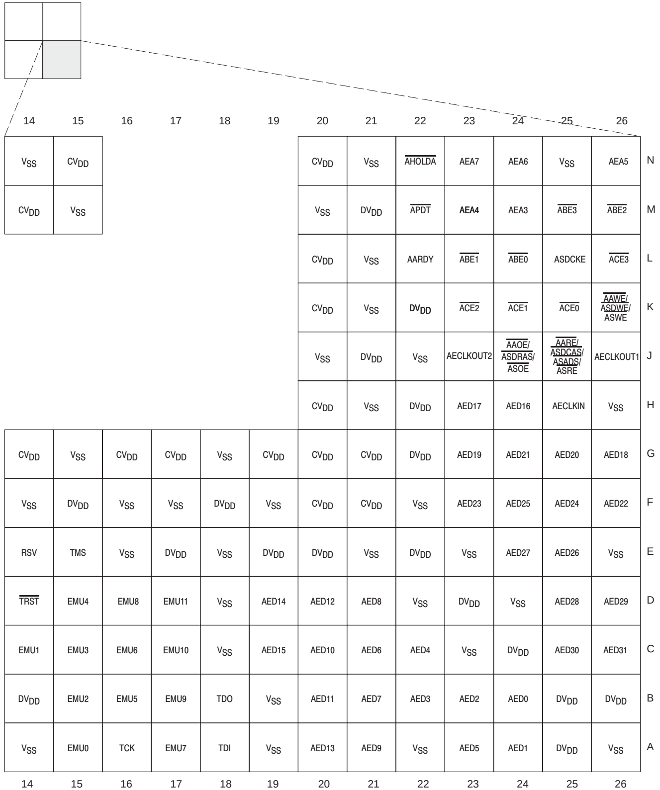
Figure 1-4. DM642 Pin Map (Continued) [Quadrant D]
