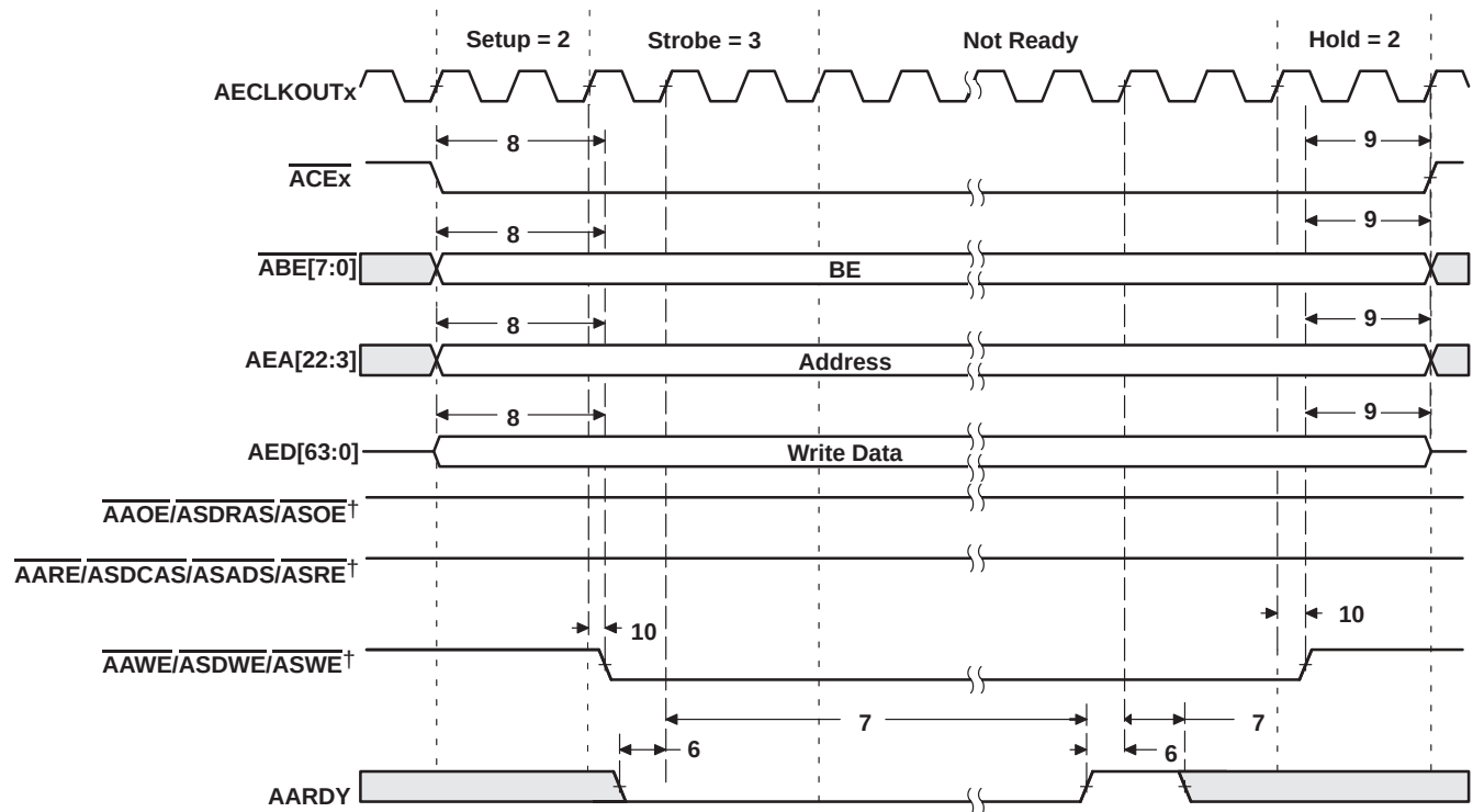
Figure 4-18. Asynchronous Memory Write Timing for EMIFA
