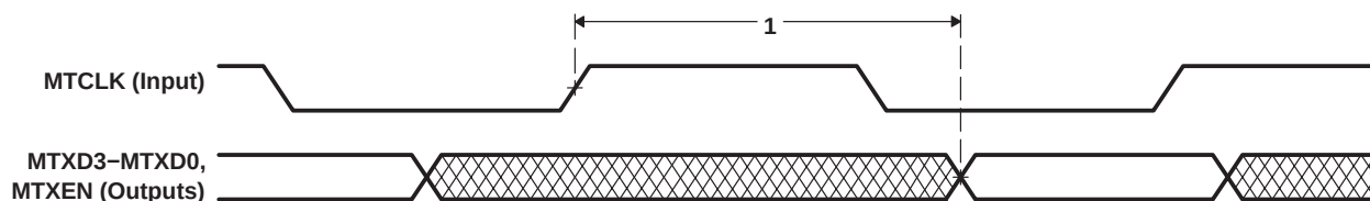
Figure 4-66. EMAC Transmit Interface Timing
