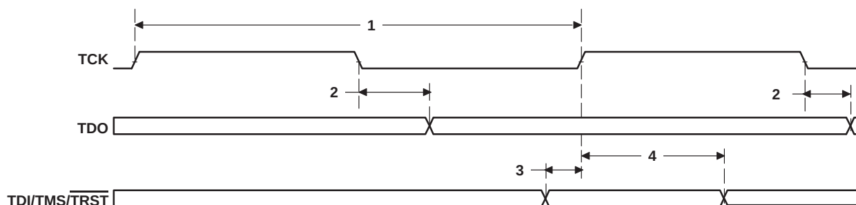
Figure 4–74. JTAG Test-Port Timing
