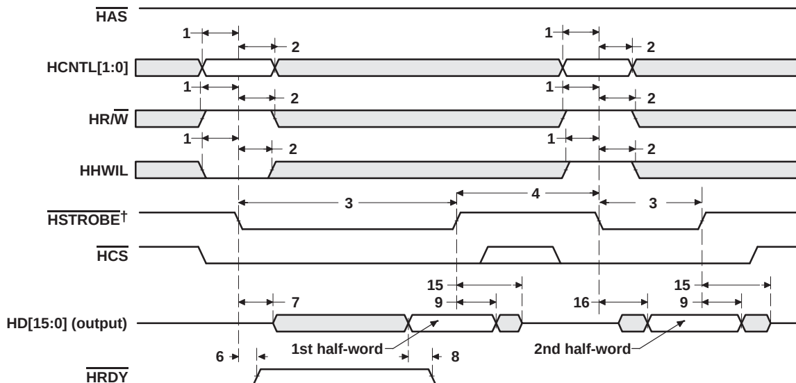
Figure 4–38. HPI16 Read Timing ( \overline{\text{HAS}} Not Used, Tied High)
