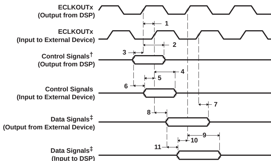
Figure 4–4. Board-Level Input/Output Timings
