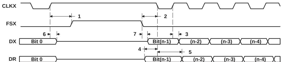
Figure 4–56. McBSP Timing as SPI Master or Slave: CLKSTP = 11b, CLKXP = 1
