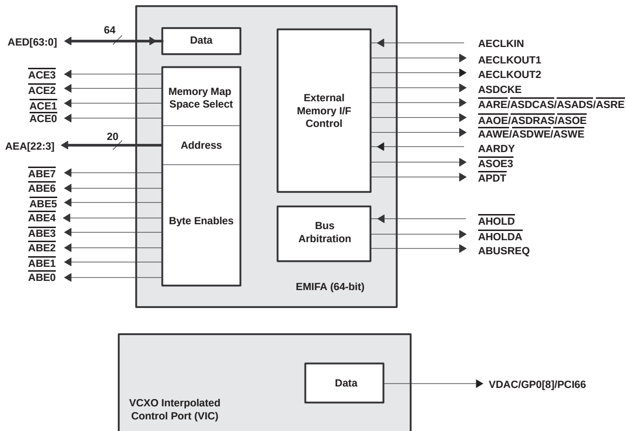
Figure 1–6. Peripheral Signals
