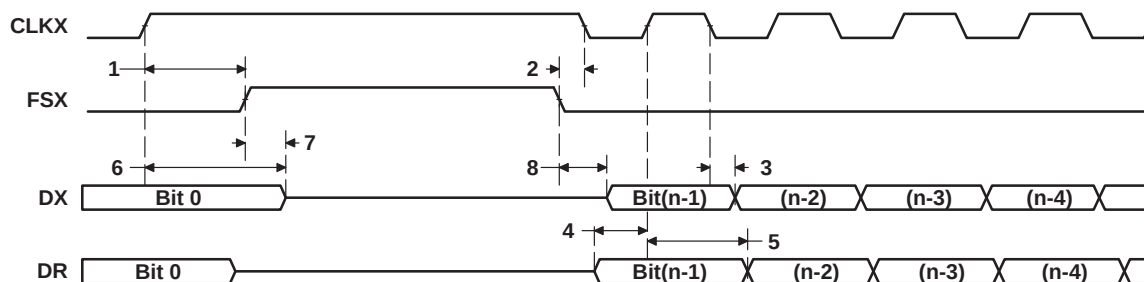
Figure 4–55. McBSP Timing as SPI Master or Slave: CLKSTP = 10b, CLKXP = 1
