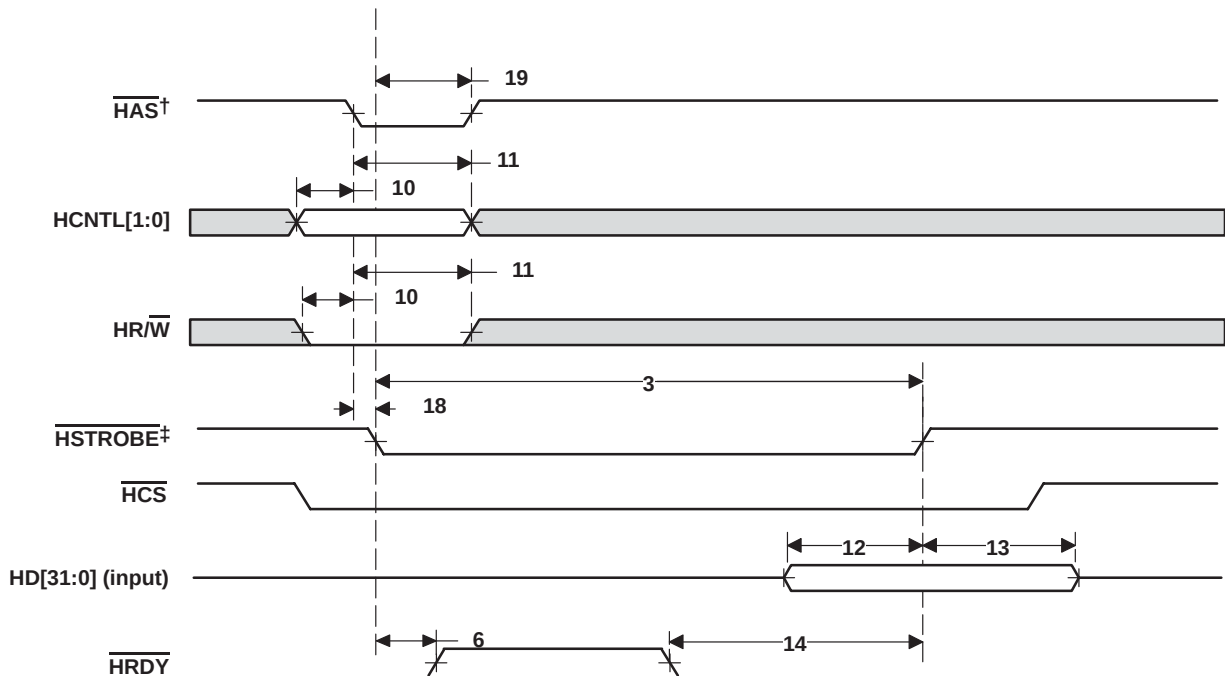
Figure 4–45. HPI32 Write Timing ( \overline{\text{HAS}} Used)
