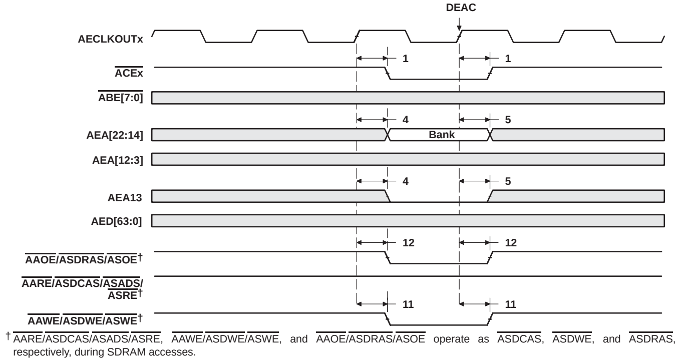
Figure 4-26. SDRAM DEAC Command for EMIFA
