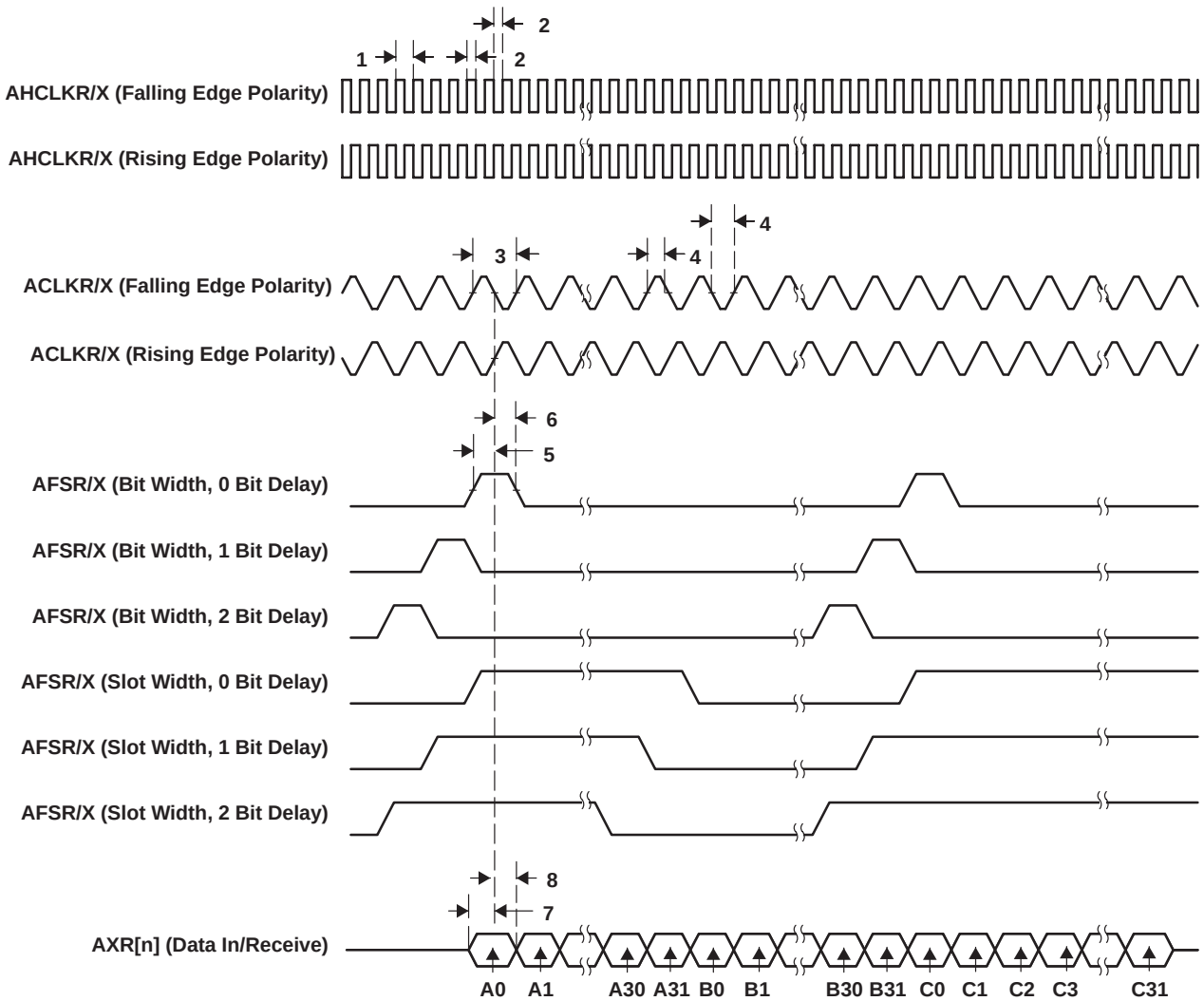
Figure 4-33. McASP Input Timings
