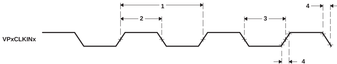
Figure 4–59. Video Port Display VPxCLKINx Timing
