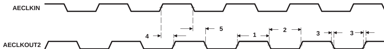
Figure 4–16. AECLKOUT2 Timing for the EMIFA Module
