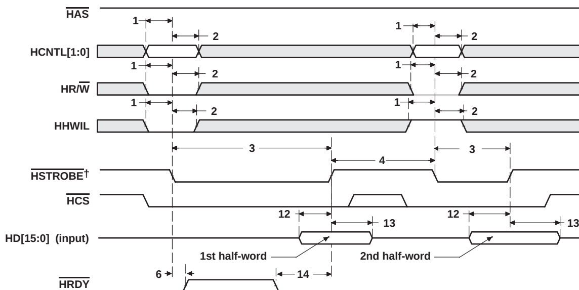
Figure 4-40. HPI16 Write Timing ( \overline{\text{HAS}} Not Used, Tied High)
