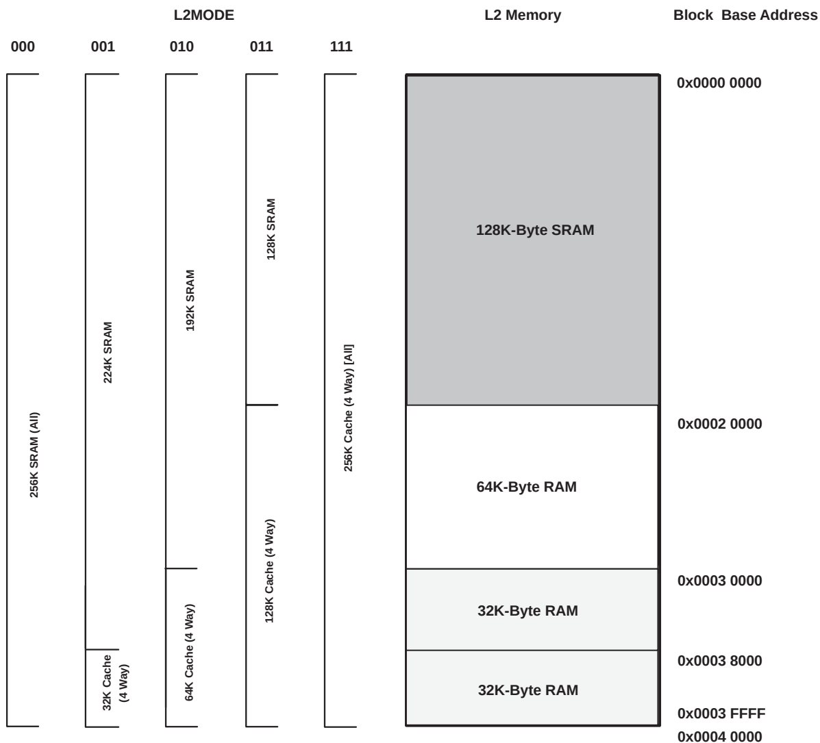
Figure 1–3. TMS320DM642 L2 Architecture Memory Configuration
