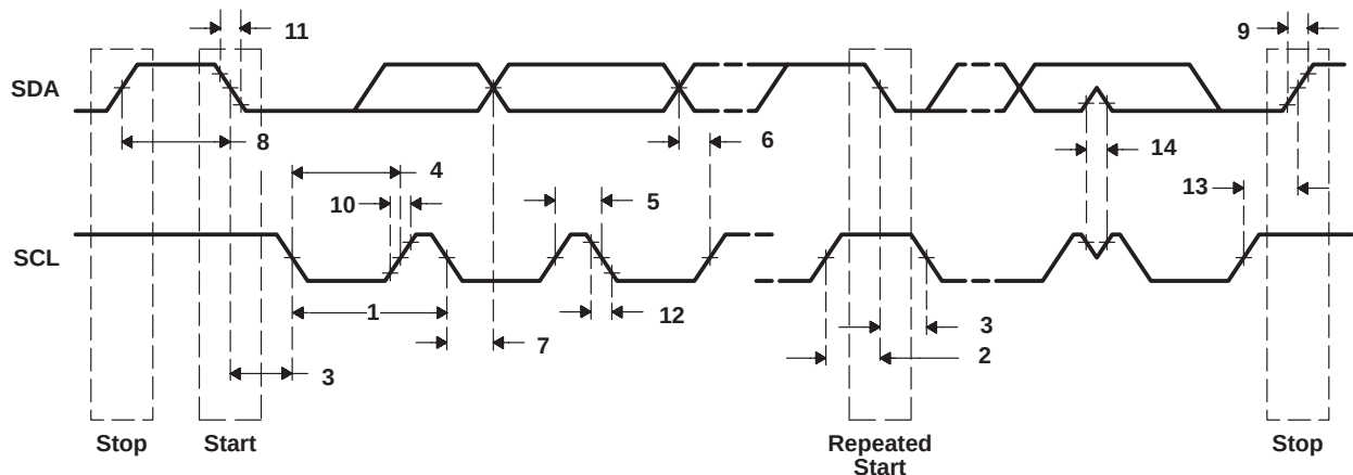
Figure 4–36. I2C Receive Timings
