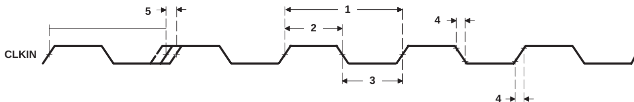
Figure 4-11. CLKIN Timing
