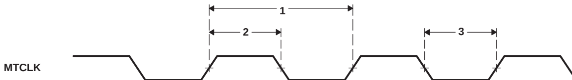
Figure 4–64. MTCLK Timing (EMAC – Transmit)
