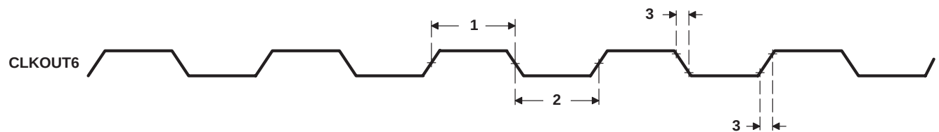
Figure 4–13. CLKOUT6 Timing
