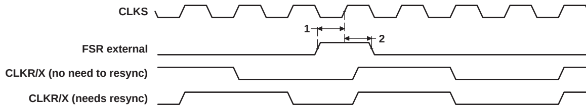
Figure 4-52. FSR Timing When GSYNC = 1
