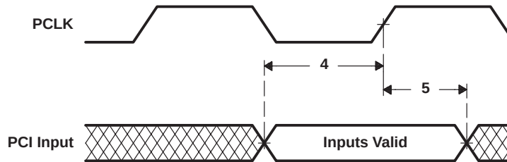
Figure 4-48. PCI Input Timing (33-/66-MHz)
