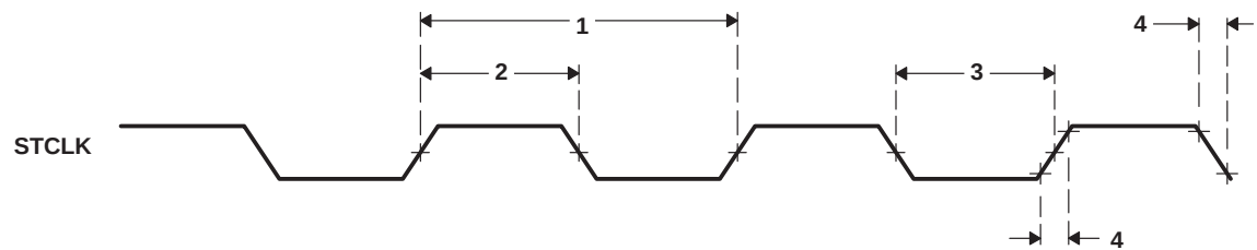
Figure 4–62. STCLK Timing
