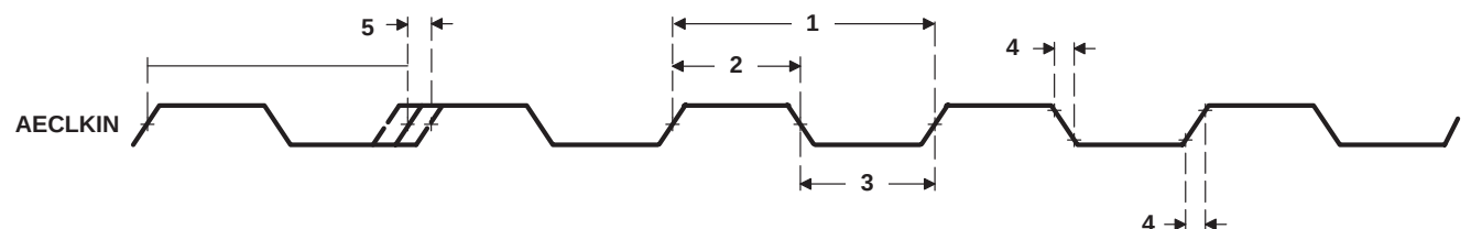
Figure 4–14. AECLKIN Timing for EMIFA
