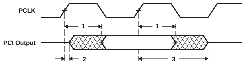
Figure 4-49. PCI Output Timing (33-/66-MHz)
