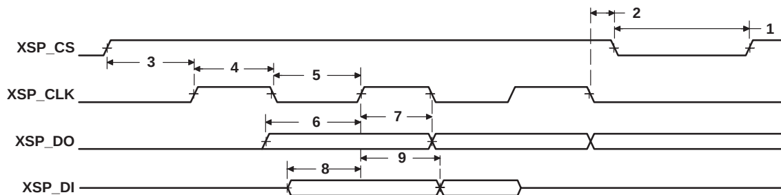
Figure 4–50. PCI Serial EEPROM Interface Timing
