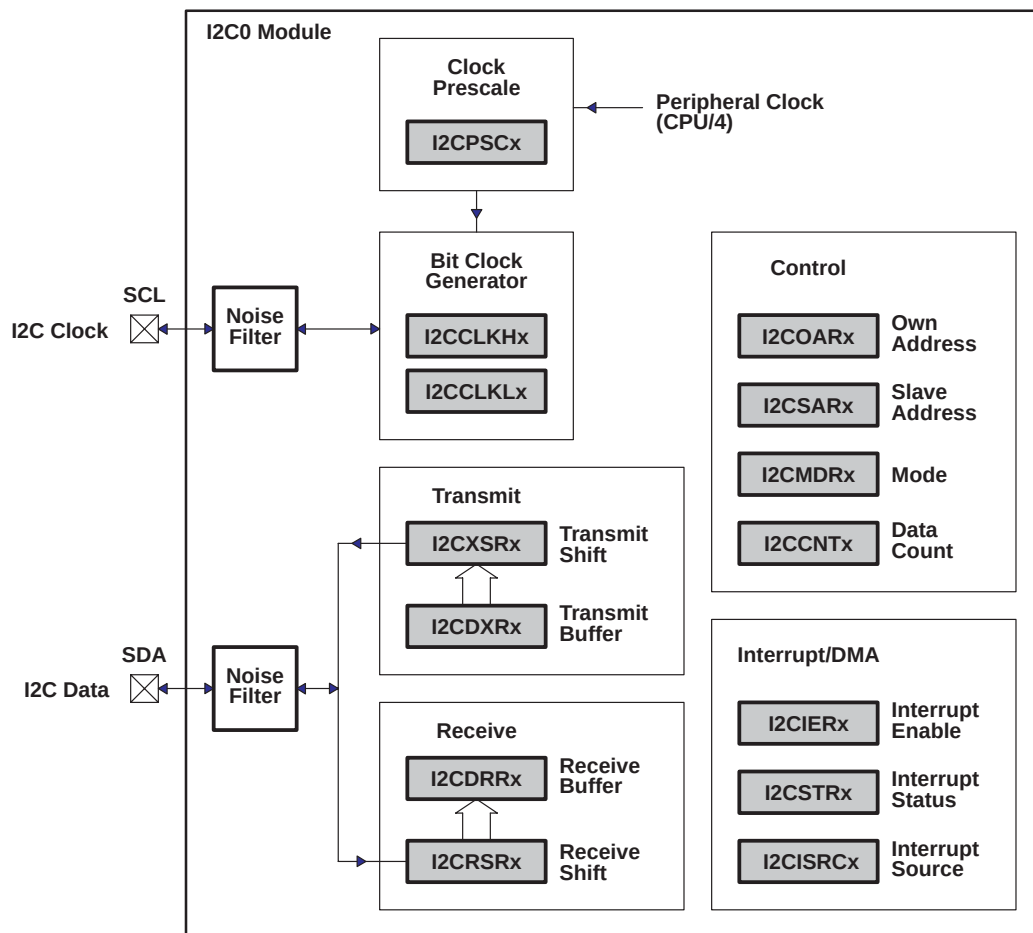
Figure 4–35. I2C0 Module Block Diagram
