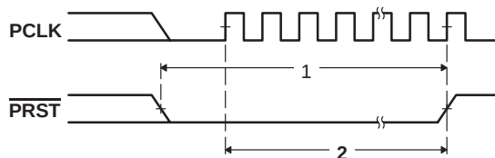
Figure 4-47. PCI Reset ( \overline{\text{PRST}} ) Timing
