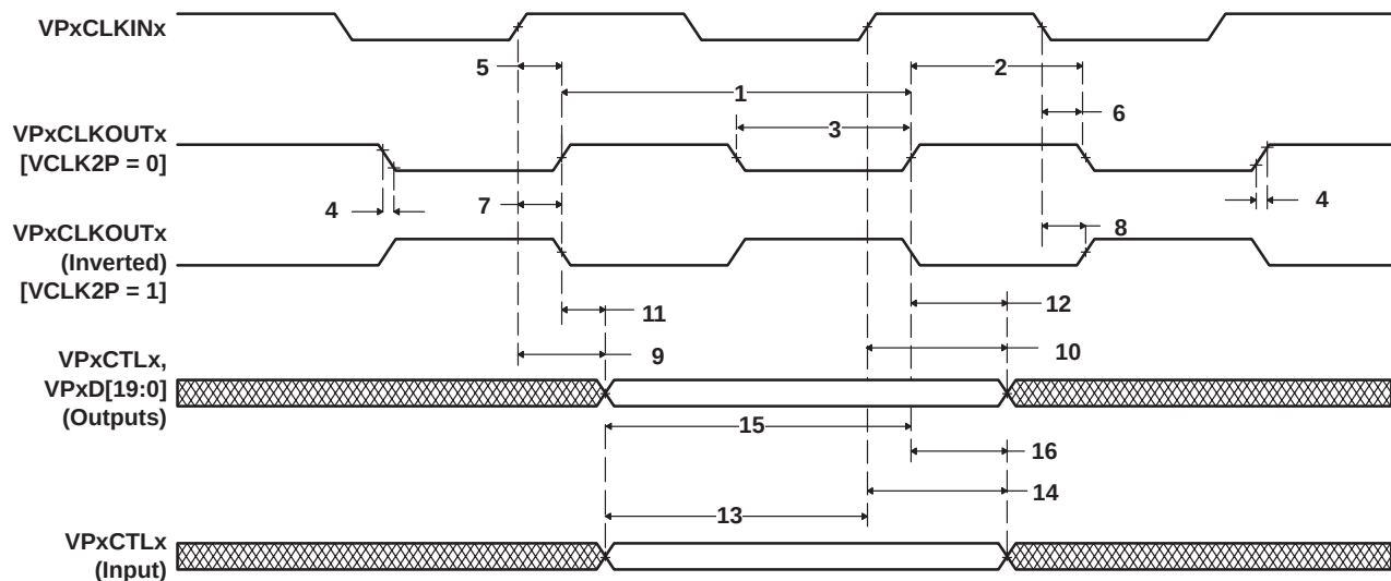
Figure 4–60. Video Port Display Data Output Timing and Control Input/Output Timing With Respect to VPxCLKINx and VPxCLKOUTx
