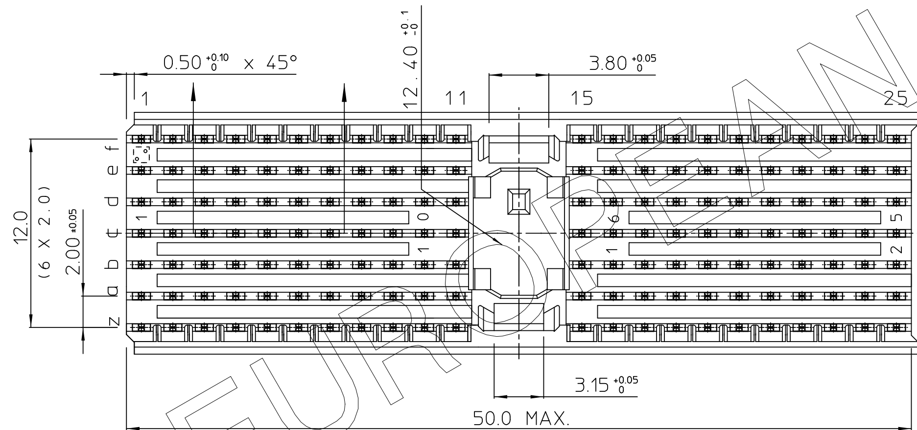
CONTACT LAY-OUT
