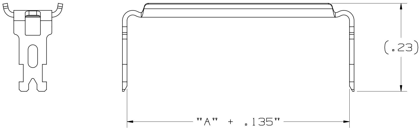
ACCESSORY - STRAIN RELIEF PART NUMBER 3448-451XX
