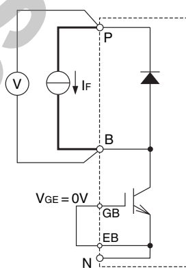
Br Di V_{GE} = 0V (GuP-EuP, GvP-EvP, GwP-EwP, GuN-EuN, GvN-EvN, GwN-EwN)
