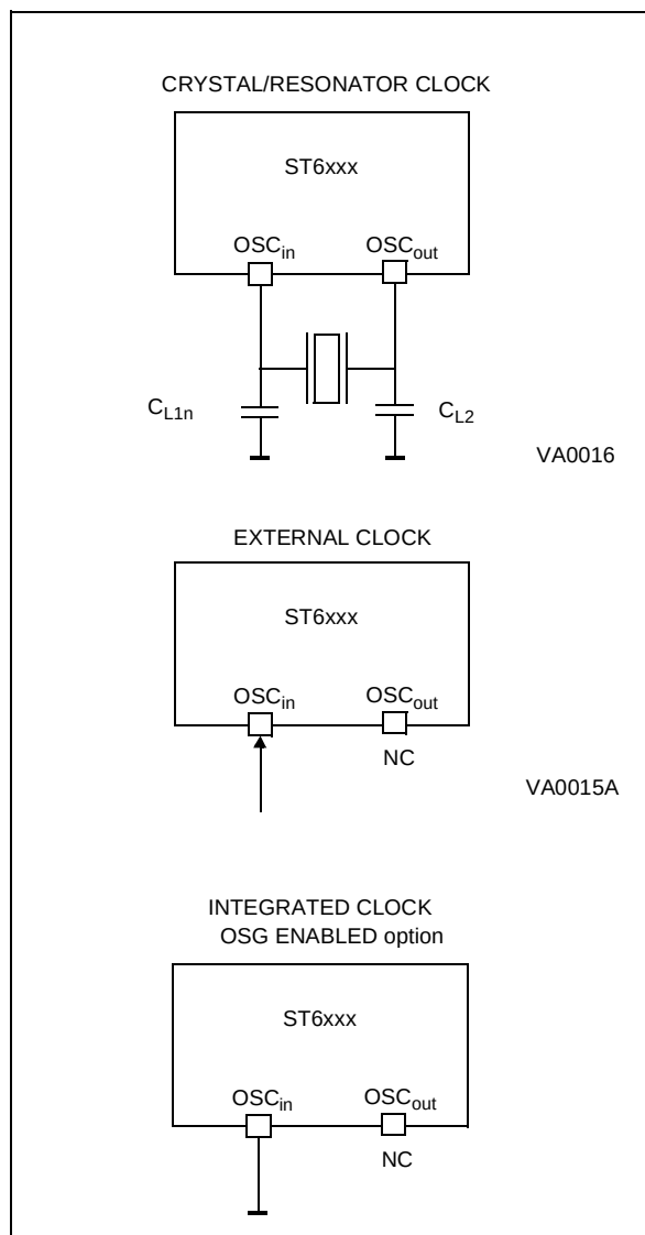
Figure 8. Oscillator Configurations
