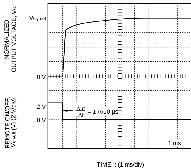
Figure 10. Typical DW025-Series Output Voltage Rise Time with Remote On/Off at V_i = V_{i,nom} , I_o = 0.8 (I_{o,max}) and T_A = 25\text{ }^{\circ}\text{C}
