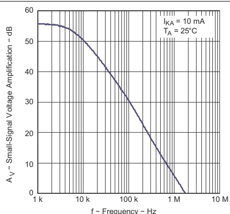
Figure 6-10. Small-Signal Voltage Amplification vs Frequency
