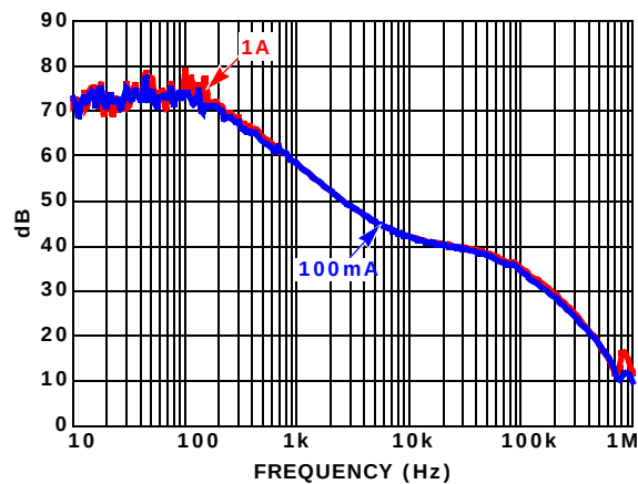
FIGURE 32. PSRR vs LOAD
