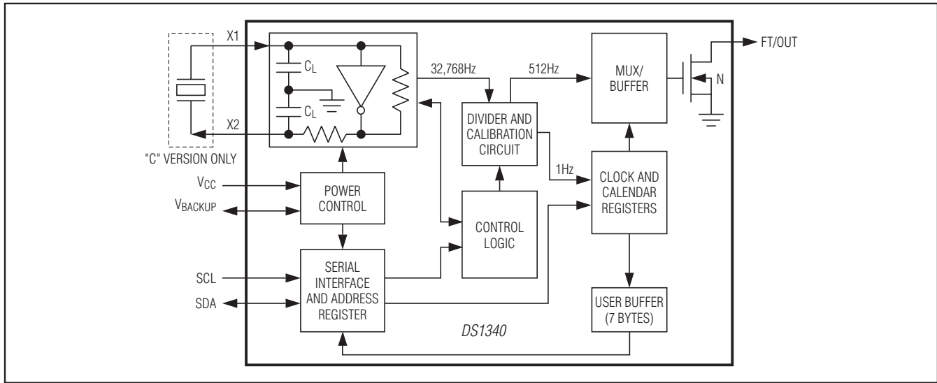
Figure 5. Functional Diagram
