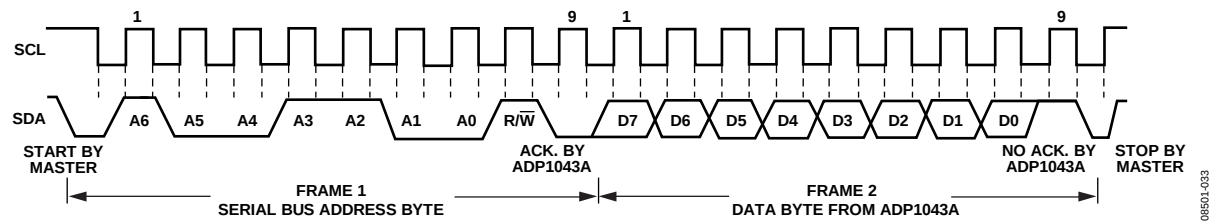
Figure 34. Reading Data from a Previously Selected Register
