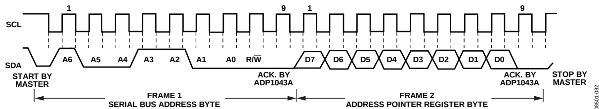
Figure 33. Writing to the Address Pointer Register Only
