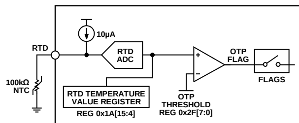
Figure 28. RTD Pin Internal Details
