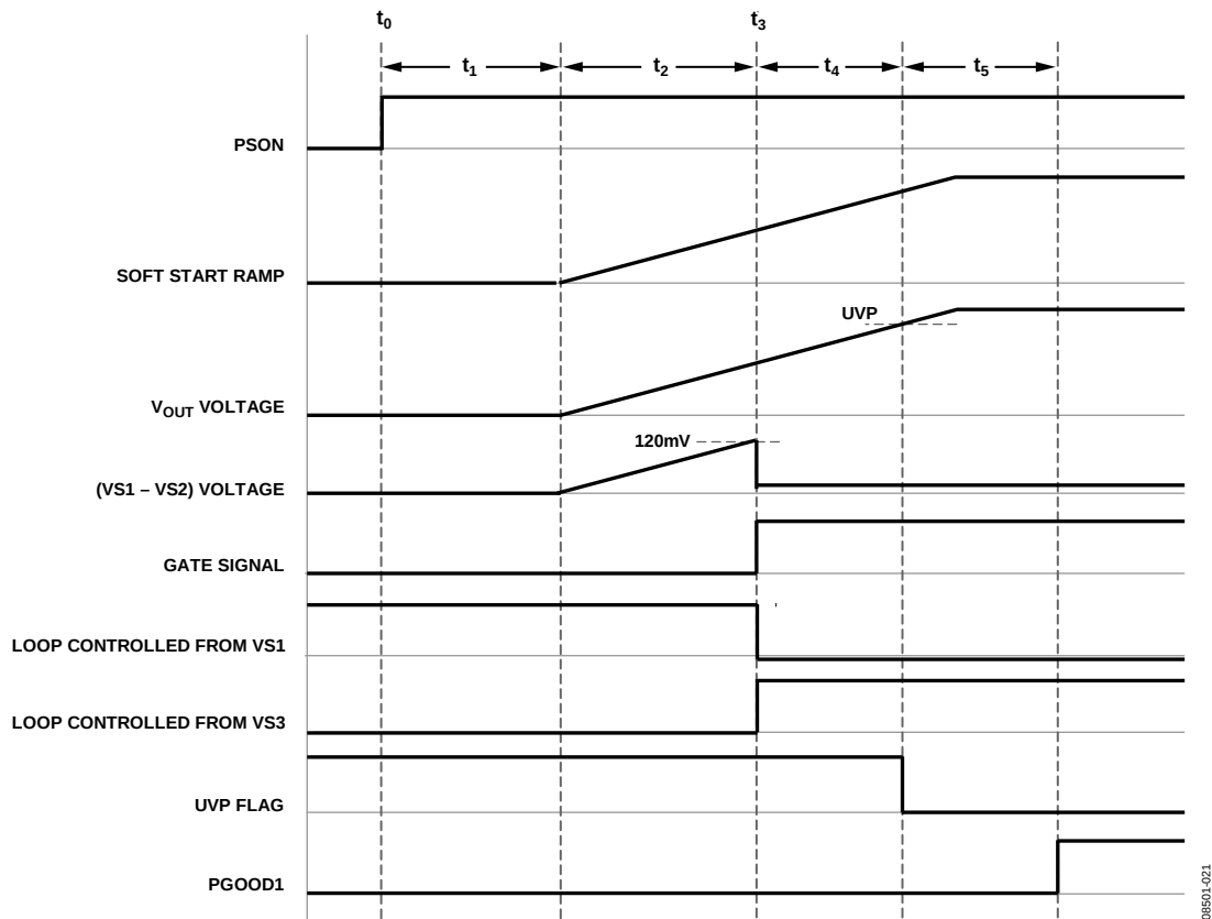
Figure 21. Soft Start Timing Diagram
