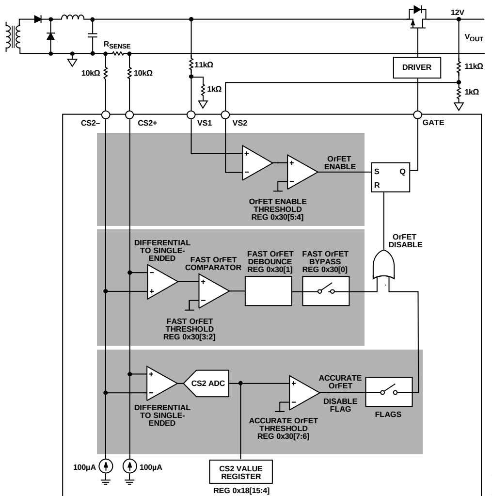
Figure 16. OrFET Control Circuit Internal Detailed Diagram
