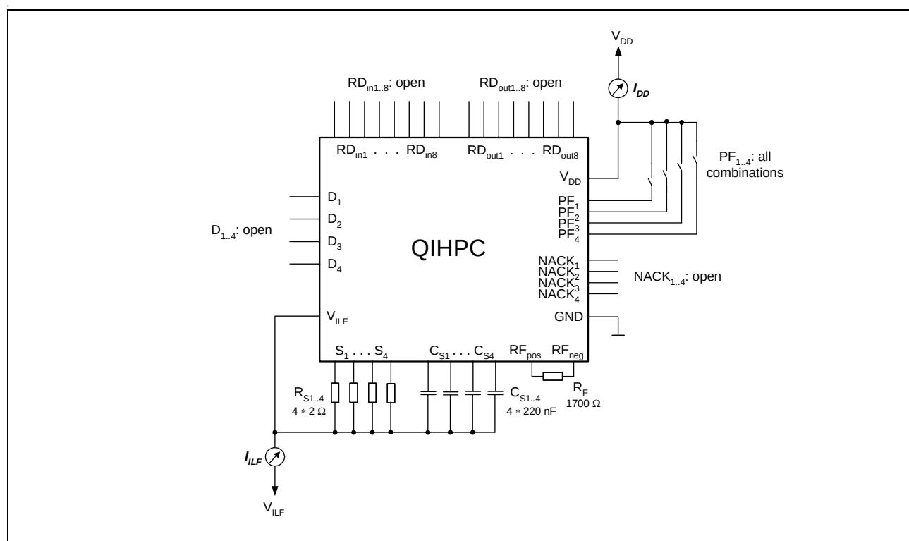
Figure 10 Supply Currents
