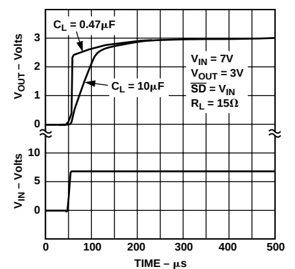
Figure 10. Power-Up Response
