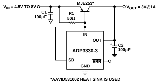
Figure 25. High Output Current Linear Regulator
